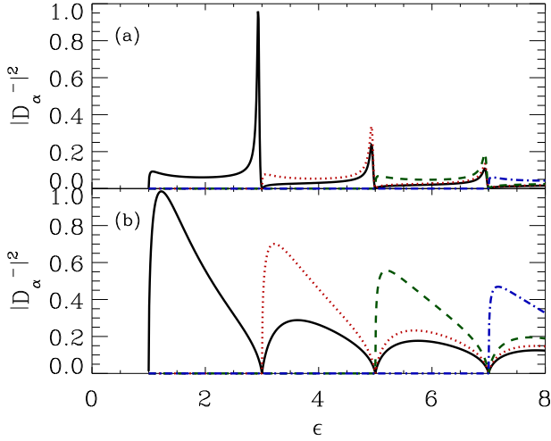
FIG. 9. (Color online) The partial absorption probability, |D_{\alpha}^{-}|^2 (in arbitrary units) for a harmonic-oscillator confining potential in arbitrary units as a function of the scaled energy, \epsilon = E/(\hbar\omega_{\perp}) . The lines are calculations using Eq. (40) with (\ell, m) = (0, 0) . Panels (a) and (b) correspond to s -wave scattering lengths of -a_{\perp}/4 and a_{\perp}/4 , respectively. The black solid line is for absorption into the first open channel, the red dotted line is second open channel, the green dashed line is third open channel, and the blue dot-dashed line is fourth open channel.
