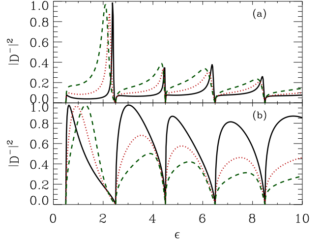
FIG. 10. (Color online) The total absorption probability |D^{-}|^2 (in arbitrary units) for an infinite square-well confining potential in arbitrary units as a function of the scaled energy \epsilon = E/(4\hbar^2\pi^2/[2\mu a_{\perp}^2]) , with (\ell, m) = (0, 0) . The lines refer to calculations based on Eq. (40). In panel (a) the s -wave scattering lengths acquire the values -a_{\perp}/16 (black solid line), -a_{\perp}/8 (red dotted line), and -a_{\perp}/4 (green dashed line). In panel (b) the s -wave scattering lengths have the values a_{\perp}/16 (black solid line), a_{\perp}/8 (red dotted line), and a_{\perp}/4 (green dashed line).
