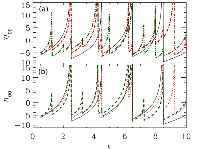
FIG. 7. (Color online) The parameter \eta_{00} for infinite square-well confinement is shown as a function of the scaled energy \epsilon = E/(4\hbar^2 \pi^2/[2\mu a_\perp^2]) with the scattering center at the scaled position (\tilde{x}_s, \tilde{y}_s) . Panel (a) (0.0, 0.0) is the black solid line, (0.1, 0.1) is the red dot-dashed line, and (0.2, 0.2) is the green dot-dot-dot-dashed line. Panel (b) (0.0, 0.0) is the black solid line, (0.1, 0.0) is the red dotted line, and (0.2, 0.0) is the green dashed line. The solid line is the same result as in Fig. 4.
