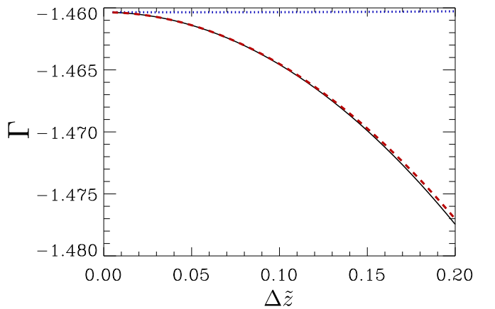
FIG. 1. (Color online) The quantity \Gamma of Eq. (32) as a function of \Delta z/a_\perp for the confining potential of the harmonic oscillator infinitesimally above the threshold energy E = \hbar\omega_\perp , where \boldsymbol{\rho}_1 = \boldsymbol{\rho}_2 = 0 . The black solid line denotes the sum in Eq. (C3). The red dashed line depicts the approximation Eq. (32) using Eq. (44). The blue dotted line indicates a numerical extrapolation of \Gamma(\mathbf{r}_1, \mathbf{r}_2, E) \equiv \Gamma(\Delta \tilde{z} \rightarrow 0^+, \Delta \tilde{\rho} \rightarrow 0, E) \simeq [4\Gamma(\Delta \tilde{z}, 0, E) - \Gamma(2\Delta \tilde{z}, 0, E)]/3 .
