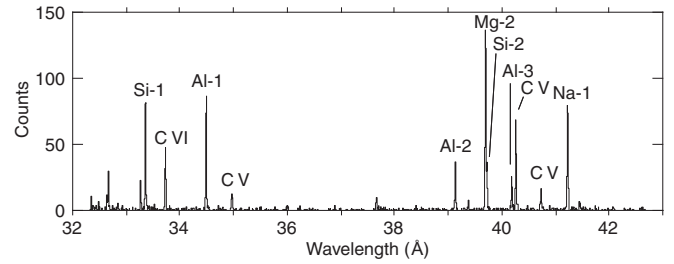
FIG. 2. EUV spectrum of Eu recorded with a flat-field spectrometer at an electron-beam energy of about 8 keV. The spectrum shows n = 3 to n' = 3 lines from sodiumlike, magnesiumlike, aluminumlike, and siliconlike ions as the strongest ones of europium, as well as calibration lines of hydrogenlike and heliumlike ions of carbon. The labels C V and C VI refer to K -shell transitions in heliumlike and hydrogenlike carbon, respectively; other labels are those used in Table I.
