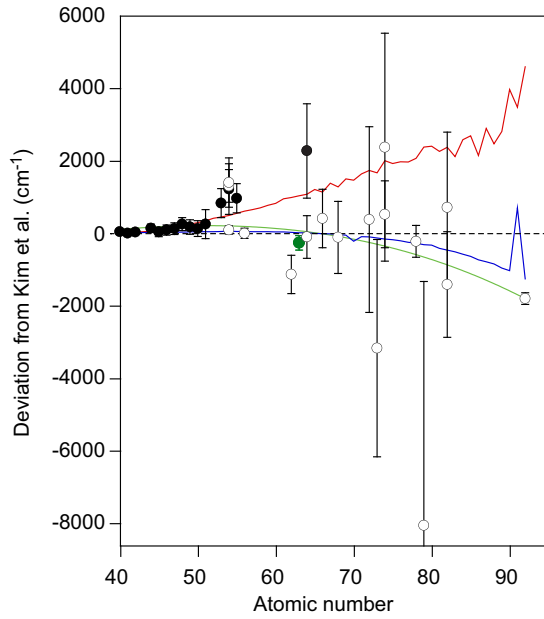
FIG. 1. (Color online) Comparison of measured and calculated energies of the 3s_{1/2}-3p_{3/2} transition in sodiumlike ions (from Z = 40 to 92). All values are relative to semiempirical values given by Kim et al. [2]. Other calculations are semiempirical calculations by Seely et al. [4] (solid red line) and ab initio calculations by Blundell [7,12] (solid blue line). The experimental data points (solid black circles) with Z \leq 50 are from a compilation by Reader et al. [16]. Data with Z \geq 53 from Refs. [4–6,8–14] are shown as solid black circles, if measured before the measurement of \text{Pt}^{67+} by Cowan et al. [5], and as open black circles otherwise. The present measurement is shown as a solid green circle. The weighted fit to all data is shown as a green line.
