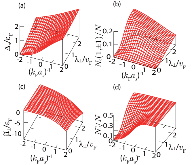
FIG. 5. (Color online) (a) Calculated s -wave superfluid order parameter \Delta_s and (c) effective chemical potential \tilde{\mu}_\perp = \mu + m\lambda_\perp^2/2 at T = 0 in the case of two-component spin-orbit interaction ( \lambda_\perp \neq 0, \lambda_z = 0 ). (b) p -wave condensate fraction N_c(S = 1, S_z = \pm 1) . (d) Total condensate fraction N_c^t .
