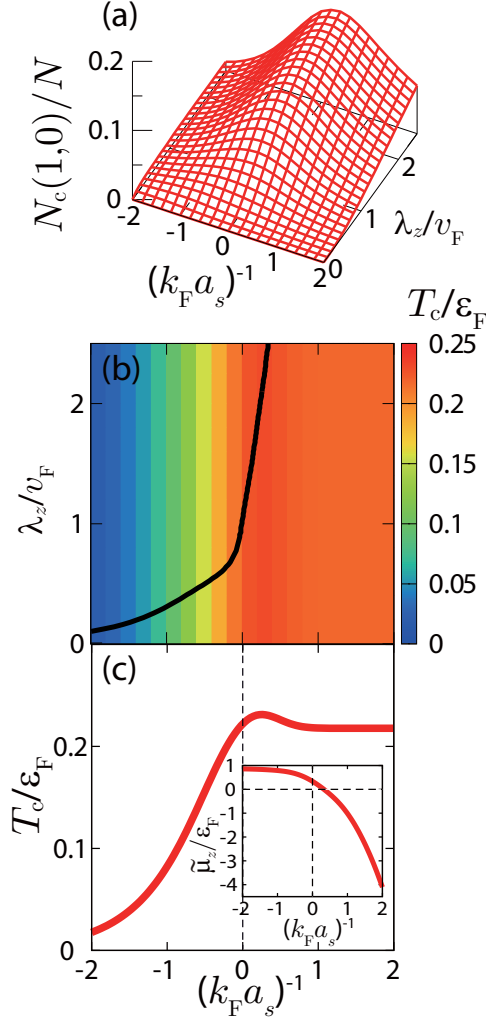
FIG. 3. (Color online) (a) Calculated p -wave condensate fraction N_c(S=1, S_z=0) at T=0 in the case of single-component spin-orbit interaction ( \lambda_\perp=0 ). (b) Peak position of N_c(S=1, S_z=0) evaluated from the result shown in panel (a). The background intensity shows T_c . (c) Calculated T_c . The inset shows the effective Fermi chemical potential \tilde{\mu}_z = \mu + m\lambda_z^2/2 .
