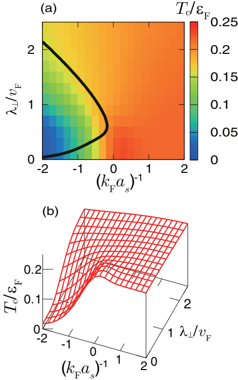
FIG. 6. (Color online) (a) Peak position of p -wave condensate fraction N_c(S=1, S_z=\pm 1) at T=0 in the case of two-component spin-orbit interaction. The background intensity represents the magnitude of T_c . For convenience, we also show the three-dimensional plot of T_c in panel (b).
