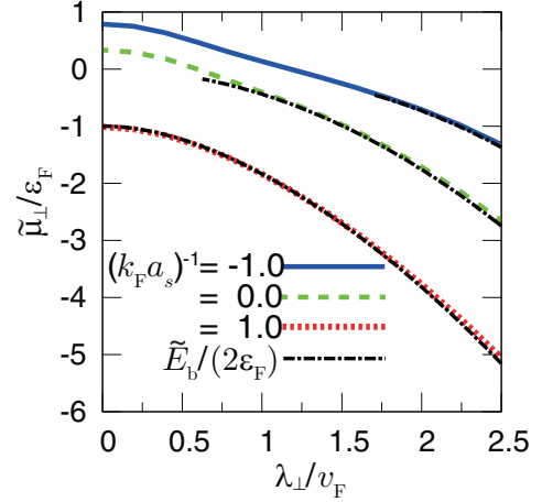
FIG. 7. (Color online) Calculated effective chemical potential \tilde{\mu}_\perp = \mu + m\lambda_\perp^2/2 at T_c as a function of the spin-orbit-coupling strength \lambda_\perp . \tilde{E}_b/2 = E_b/2 + m\lambda_\perp^2/2 , where E_b is the binding energy of a two-body bound state, determined from Eq. (44).
