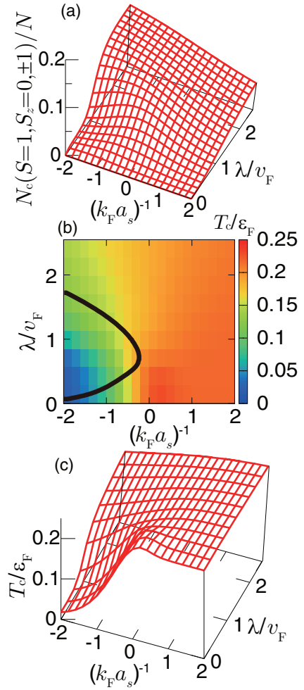
FIG. 9. (Color online) (a) p -wave condensate fraction N_c(S = 1, S_z = 0, \pm 1) at T = 0 in the case of isotropic spin-orbit interaction \lambda_\perp = \lambda_z = \lambda/\sqrt{2} ( \theta_\lambda = \pi/4 ). (b) Peak position of N_c(S = 1, S_z = 0, \pm 1) evaluated from panel (a). The background intensity shows T_c , which is also shown in panel (c) for clarity.
