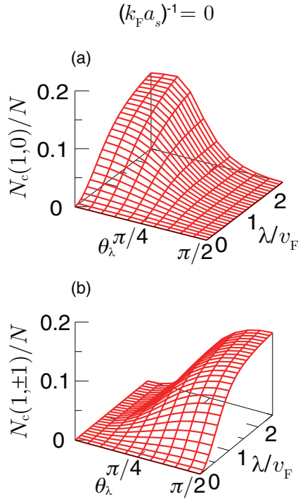
FIG. 8. (Color online) Calculated p -wave condensate fraction at T = 0 in the case of three-component spin-orbit interaction (\lambda_\perp, \lambda_z) = \lambda(\sin \theta_\lambda, \cos \theta_\lambda) . We set (k_F a_s)^{-1} = 0 . (a) N_c(S = 1, S_z = 0) . (b) N_c(S = 1, S_z = \pm 1) . In this figure, \theta_\lambda = 0 and \theta_\lambda = \pi/2 , respectively, correspond to the single-component and two-component spin-orbit interaction, discussed in the previous subsections.
