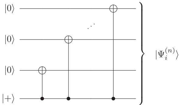
FIG. 1. Quantum circuit to initialize the n system qubits. The qubits are prepared in the maximally entangled state |\Psi_i\rangle = (|0\rangle^{\otimes n} + |1\rangle^{\otimes n})/\sqrt{2} by a sequence of CNOT gates.
