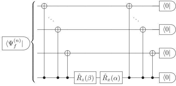
FIG. 3. Quantum circuit to postselect the n system qubits in the entangled state |\Psi_f\rangle [Eq. (66)], which is in essence the reverse process of preparing |\Psi_f\rangle from |0\rangle^{\otimes n} .
