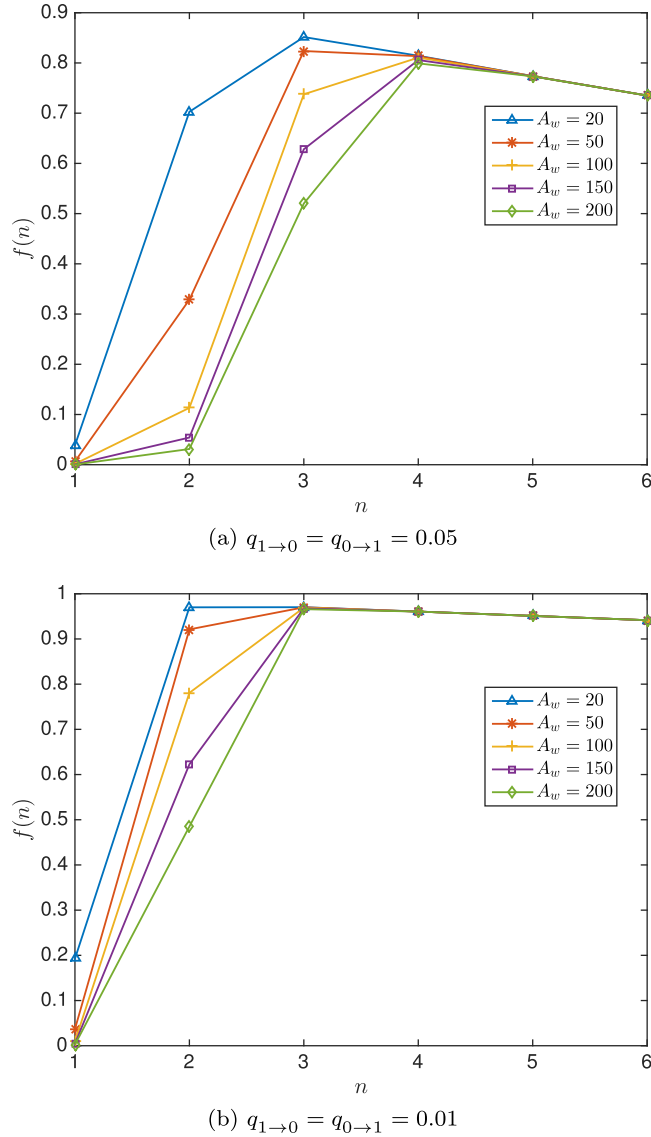
FIG. 8. (Color online) This figure plots the modification factor f(n) of the Fisher information versus the number of entangled qubits n in the presence of readout errors, but without majority voting, for different weak values. When n is small, the Fisher information can increase with n because the entanglement eliminates some errors in the postselection results and raises the proportion of correct postselected states that have higher Fisher information. However, when n becomes larger, the Fisher information starts to fall since the loss rate of correct postselected states dramatically increases with n in this case.
