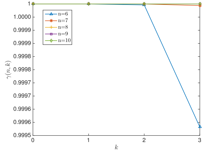
(b) q_{1 \rightarrow 0} = q_{0 \rightarrow 1} = 0.01
