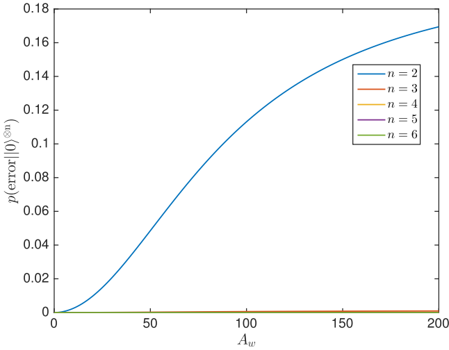
(b) q_{1 \rightarrow 0} = q_{0 \rightarrow 1} = 0.01
