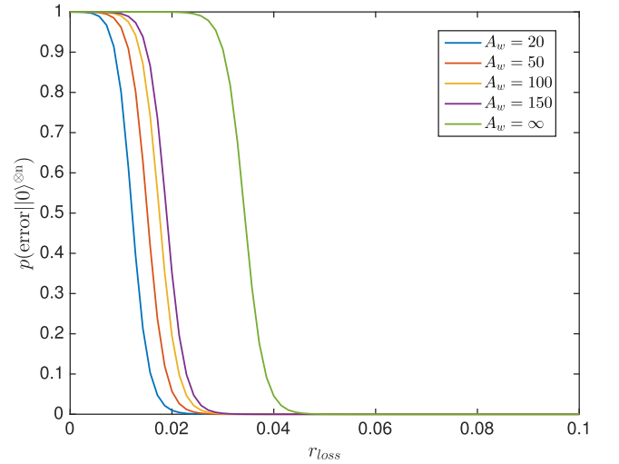
(b) q_{1 \rightarrow 0} = q_{0 \rightarrow 1} = 0.01
