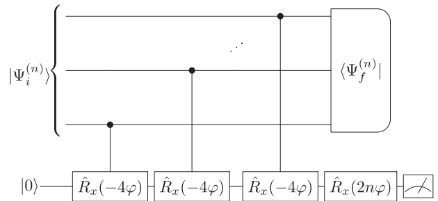
FIG. 2. Quantum circuit equivalent to the weak interaction H_{\text{int}} = \varphi \hat{\sigma}_z \otimes \hat{\sigma}_x , \varphi \ll 1 , between n system qubits and one common pointer qubit.
