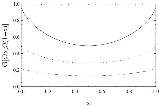
FIG. 5. Dependence of G[\Omega x, \Omega(1-x)] , Eq. (29), on x at \Omega = 0.3 (dashed curve), \Omega = 0.5 (dotted curve), and \Omega = 0.7 (solid curve). Here \Omega = (\omega_1 + \omega_2)/\varepsilon_p and x = \omega_1/(\omega_1 + \omega_2) .
