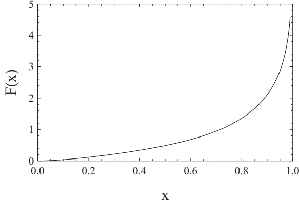
FIG. 4. Dependence of F(x) , Eq. (29), on x = \omega_1/\varepsilon_p .
