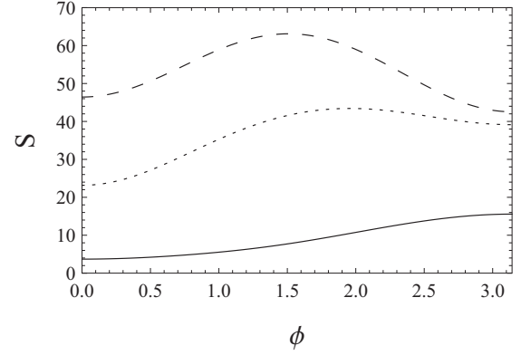
FIG. 2. The quantity S (26) as a function of the azimuth angle \phi between vectors \theta_{k_1} and \theta_{k_2} at \omega_1/\varepsilon_p = 0.2 , \omega_2/\varepsilon_p = 0.4 , \delta_1 = 0.2 , \delta_2 = 0.5 (dashed curve), \delta_2 = 1 (dotted curve), and \delta_2 = 2 (solid curve).
