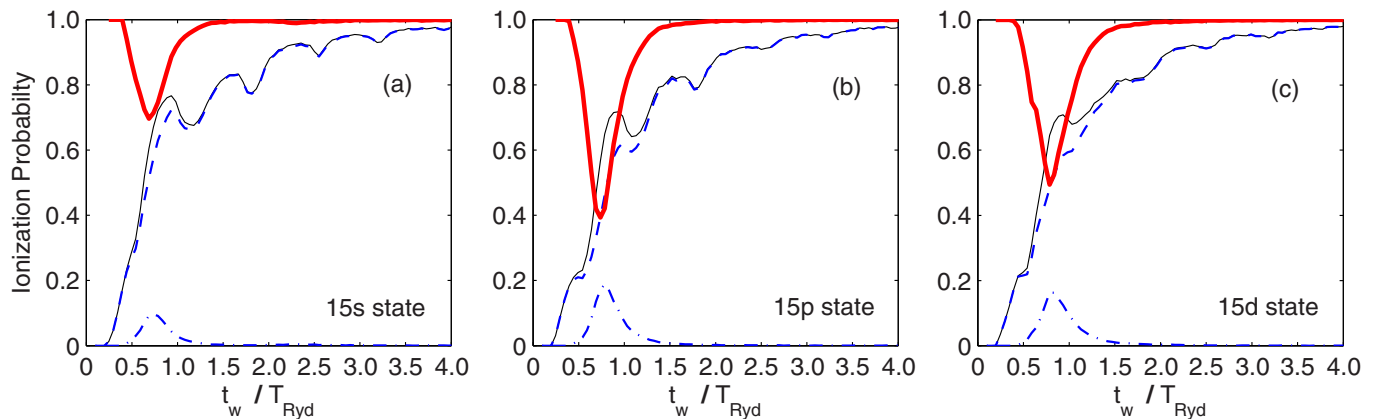
FIG. 4. (Color online) Dependence of the electron-emission asymmetry on the single-cycle pulse duration. (a)–(c) The hydrogen 15s, 15p, and 15d states, respectively. The thin black solid line shows the total ionization probability. The blue dashed and dot-dashed lines present the ionization probabilities for the electron emitted to the right side and to the left side, respectively. The asymmetry parameter \alpha_A is given by the thick red solid line.
