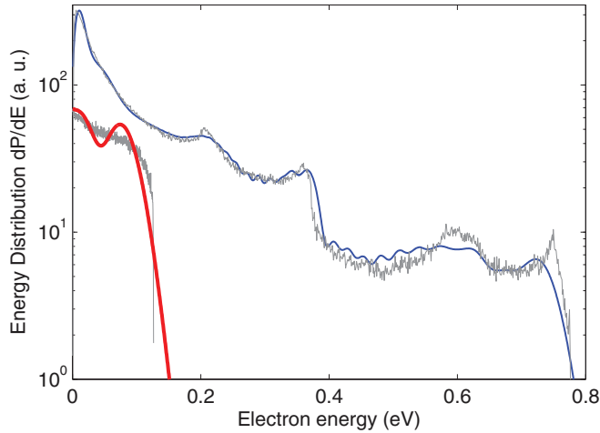
FIG. 7. (Color online) Comparison between the energy spectra from Figs. 6(a) and 6(d) on a logarithmic scale. The thin blue and thick red solid lines display the quantum spectra from Fig. 6(a) ( t_w = 0.5 ps) and Fig. 6(d) ( t_w = 0.1 ps), respectively. The corresponding spectra from CTMC calculations are shown by the thin gray curves.
