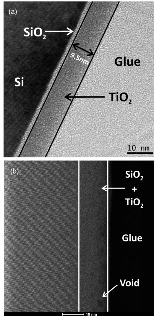
FIG. 7. (a) High-resolution TEM image of the TiO_2 film using phase contrast. (b) Scanning transmission electron microscope (STEM) image of the same sample. In (b) no difference could be observed between the contributions of TiO_2 and SiO_2 , present as a native oxide.
