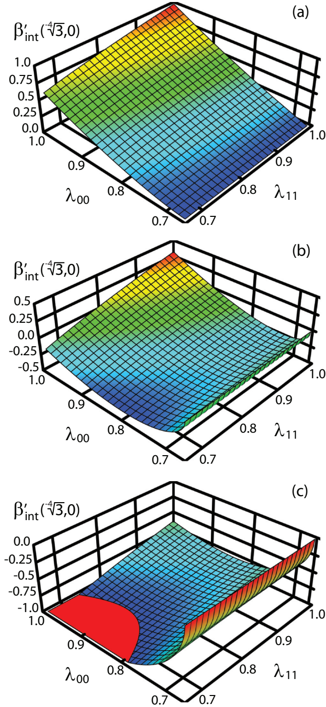
FIG. 1. (Color online) The intrinsic hyperpolarizability as a function of \lambda_{00} and \lambda_{11} when X = 1/\sqrt[4]{3} and E = 0 . The relativistic behavior of the Kuzyk limit is illustrated for (a) \lambda_{10} = 0 , (b) \lambda_{10} = 0.1 , and (c) \lambda_{10} = 0.2 . Values outside the magnitude for the nonrelativistic limit are given by the solid (red) region.
