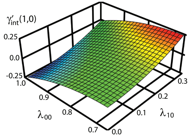
FIG. 3. (Color online) The minimum intrinsic value of the second hyperpolarizability as a function of \lambda_{00} and \lambda_{10} from the relativistic corrections to the TRK sum rules.
