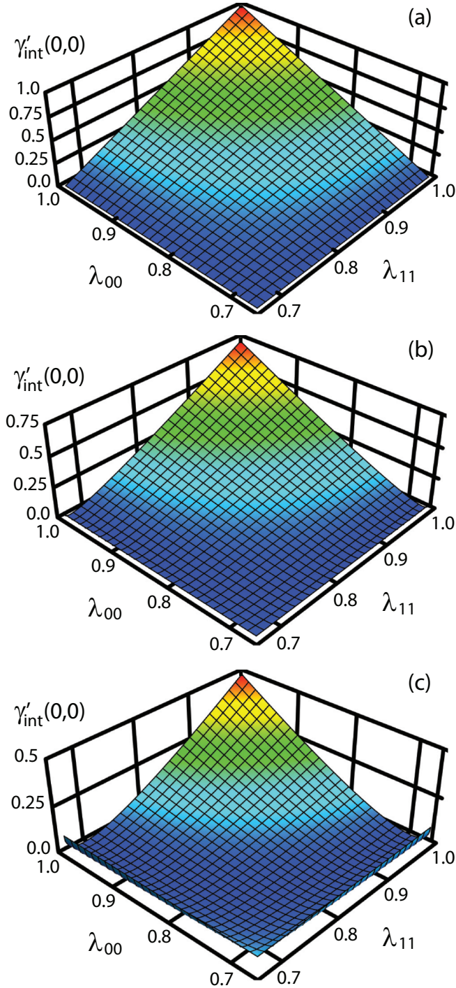
FIG. 2. (Color online) The maximum intrinsic value of the second hyperpolarizability as a function of \lambda_{00} and \lambda_{11} from the relativistic corrections to the TRK sum rules. The corrected maximum is shown for (a) \lambda_{10} = 0 , (b) \lambda_{10} = 0.1 , and (c) \lambda_{10} = 0.2 .
