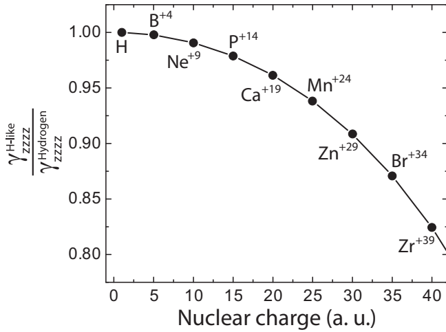
FIG. 4. The second hyperpolarizability as a function of atomic number for an H-like ion using the three-level model with lowest-order relativistic corrections to the TRK sum rules.
