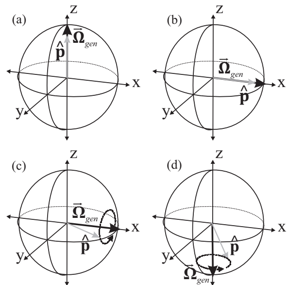
FIG. 4. Raman ARP Ramsey sequence on the Bloch sphere. (a) Following state preparation, \bar{\Omega}_{\text{gen}} is parallel to \hat{\mathbf{p}} . (b) The first sweep transfers the pseudospin polarization into the x - y plane when its center frequency matches the Raman resonance condition. (c) After a Ramsey interrogation time T , the second beamsplitter generally begins with nonparallel \bar{\Omega}_{\text{gen}} and \hat{\mathbf{p}} , which leads to precession of \hat{\mathbf{p}} about \bar{\Omega}_{\text{gen}} . (d) The second beamsplitter drags \hat{\mathbf{p}} to the z axis, mapping the relative phase between the drive field and pseudospin polarization to population difference.
