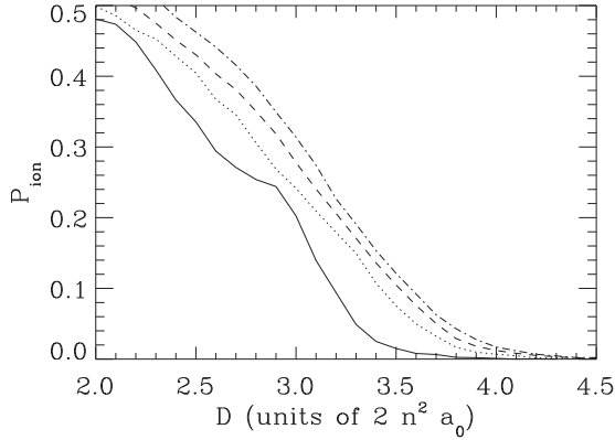
FIG. 2. The probability for ionization as a function of the atom separation for atoms in a square lattice. The different line types correspond to different number of atoms: 2^2 atoms (solid line), 3^2 atoms (dotted line), 4^2 atoms (dashed line), and 5^2 atoms (dash-dotted line).
