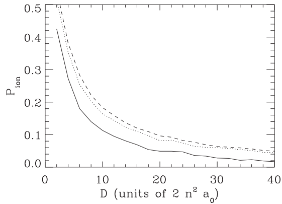
FIG. 4. The probability for ionization for atoms randomly placed on a line with the linear density 1/D . The different line types correspond to different number of atoms: 2 atoms (solid line), 4 atoms (dotted line), and 8 atoms (dashed line). Note the vastly different range for D compared to Fig. 1.
