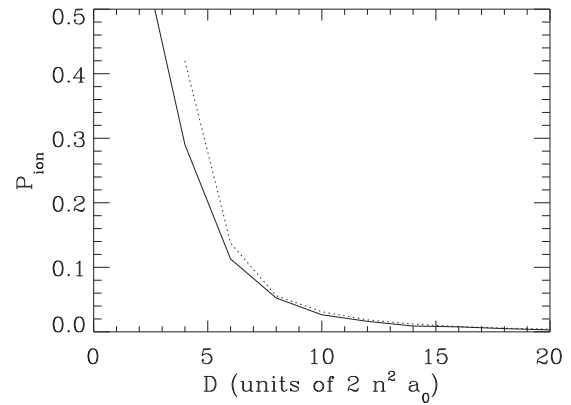
FIG. 6. The probability for ionization for atoms randomly placed within a cube with a density 1/D^3 . The different line types correspond to different number of atoms: 2^3 atoms (solid line) and 3^3 atoms (dotted line). Note the vastly different range for D compared to Fig. 3.
