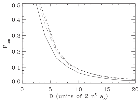
FIG. 5. The probability for ionization for atoms randomly placed within a square with the surface density 1/D^2 . The different line types correspond to different number of atoms: 2^2 atoms (solid line), 3^2 atoms (dotted line), 4^2 atoms (dashed line), and 5^2 atoms (dashed-dotted line). Note the vastly different range for D compared to Fig. 2.
