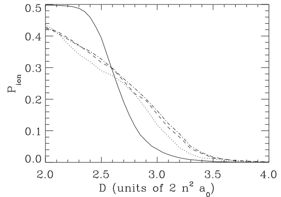
FIG. 1. The probability for an atom to be ionized as a function of the atom separation for atoms in a line. The different line types correspond to different number of atoms: 2 atoms (solid line), 4 atoms (dotted line), 8 atoms (dashed line), and 16 atoms (dashed-dotted line).
