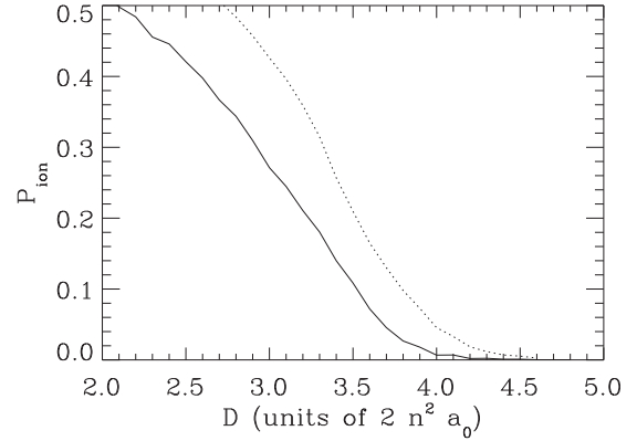
FIG. 3. The probability for ionization as a function of the atom separation for atoms in a cubic array. The different line types correspond to different number of atoms: 2^3 atoms (solid line) and 3^3 atoms (dotted line).
