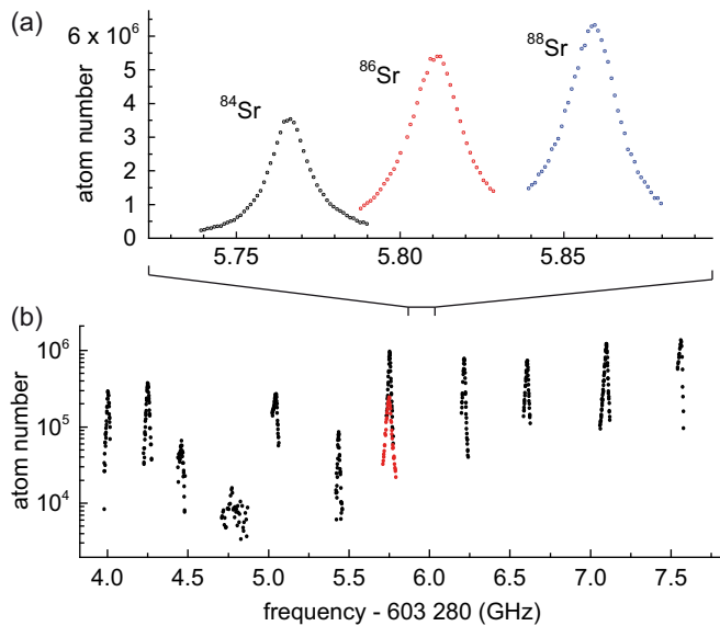
FIG. 4. (Color online) Reservoir spectroscopy data obtained with the absorption imaging detection method, shown here for the 5s5p\ ^3P_2-5s5d\ ^3D_2 transition. (a) Transitions of the bosonic isotopes ^{84}\text{Sr} (black, left peak), ^{86}\text{Sr} (red, center), and ^{88}\text{Sr} (blue, right). (b) A scan across the transitions of the fermionic ^{87}\text{Sr} isotope. The separate measurement of the two overlapping lines around 5.75 GHz is discussed in Sec. III D.
