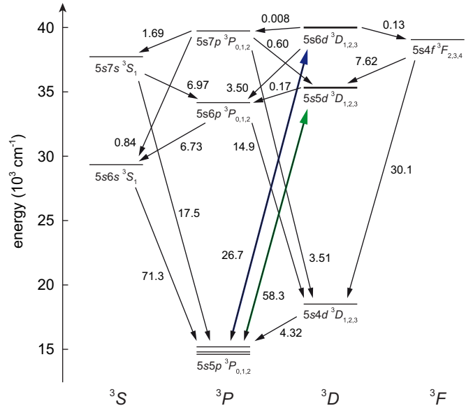
FIG. 5. (Color online) Transition probabilities A_{ik} , given in units of 10^6\text{ s}^{-1} , between triplet states of Sr relevant for this work. Values are taken from Ref. [86]. The fine structure splitting, indicated here only for the lowest ^3P_J states, is otherwise smaller than the thickness of the horizontal lines. Decay paths with negligible contribution are omitted.
