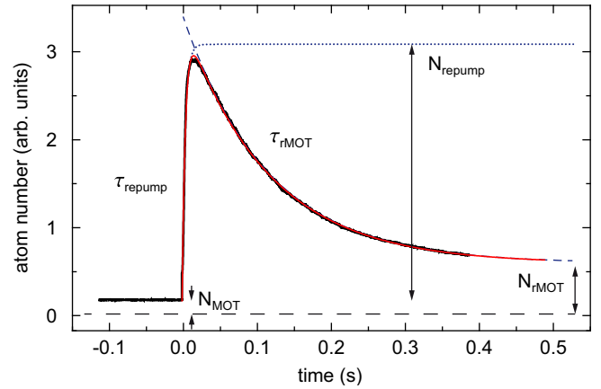
FIG. 2. (Color online) Burst in MOT fluorescence after repumping of atoms in the ^3P_2 reservoir state back into the MOT cycle. The data is approximated by the sum of two exponential functions (solid red line), consisting of a fast growing ( \tau_{\text{repump}} , dotted blue line) and a slowly decreasing contribution ( \tau_{\text{rMOT}} , dashed blue line). The horizontal dashed line indicates the small and stable background signal, caused by residual stray light.
