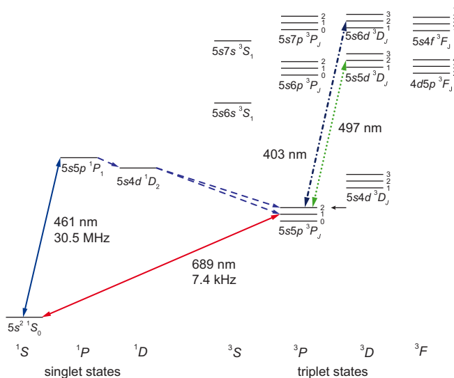
FIG. 1. (Color online) Schematic illustration of the energy levels and transitions in strontium relevant for this work. Atoms in the metastable 5s5p ^3P_2 state (indicated by the small solid arrow) are repumped using the 5s5p ^3P_2 - 5snd ^3D_{1,2,3} transitions around 497 nm ( n = 5 , dotted line) and around 403 nm ( n = 6 , dash-dotted line).
