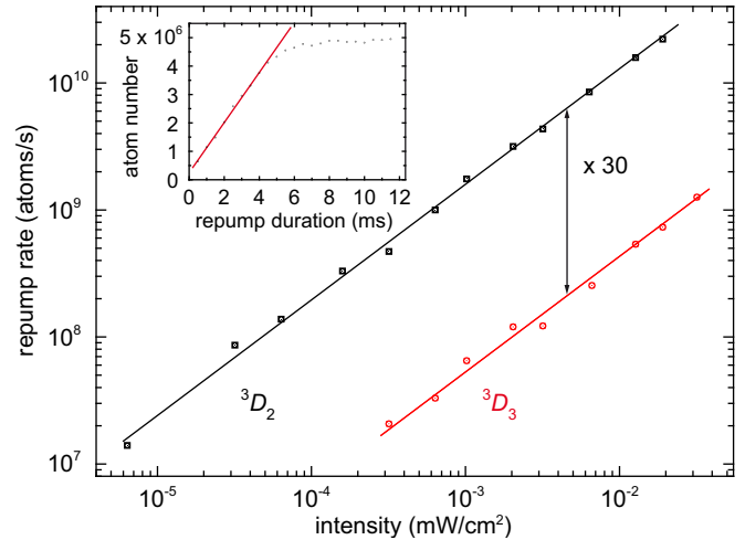
FIG. 6. (Color online) Repump rate in dependence of light intensity. The number of atoms repumped into the ^1S_0 ground state is proportional to the repump time before reaching saturation (inset, taken on the green 5s5p\ ^3P_2 - 5s5d\ ^3D_3 transition at I = 1 \times 10^{-2} I_{\text{sat}} ). This rate is measured for a large range of intensities on both of the green ^3P_2 - ^3D_2 and ^3P_2 - ^3D_3 transitions.
