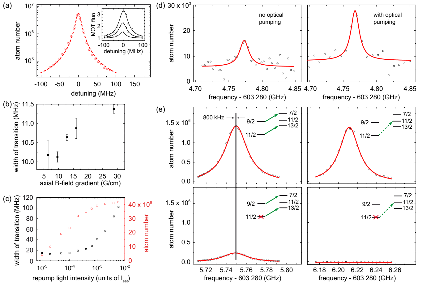
FIG. 3. (Color online) Reservoir spectroscopy scheme. (a) The reservoir spectroscopy signal is background free and rises many orders of magnitude above the background noise. By contrast, the fluorescence signal of a MOT (inset) is increased by only a small factor on resonance. A Lorentzian profile is fit to each data set, and the fluorescence curves are taken at a repump laser intensity of I = 1, 3, and 10 \times 10^{-3} I_{\text{sat}} , from below. (b) Dependence of the width of the transition on the depth of the magnetic trap. (c) Width (black squares) and atom number (red circles) in dependence of repump light intensity. The repump pulse duration is 10 ms. (d) Accumulation of a certain hyperfine state by optical pumping increases the signal. (e) Depletion of a certain hyperfine state allows for a separation of otherwise overlapping hyperfine transitions. Measurements (a) through (c) are taken on the 5s5p^3P_2-5s5d^3D_2 transition of ^{88}\text{Sr} , measurements (d) and (e) employ ^{87}\text{Sr} ; see the text for details.
