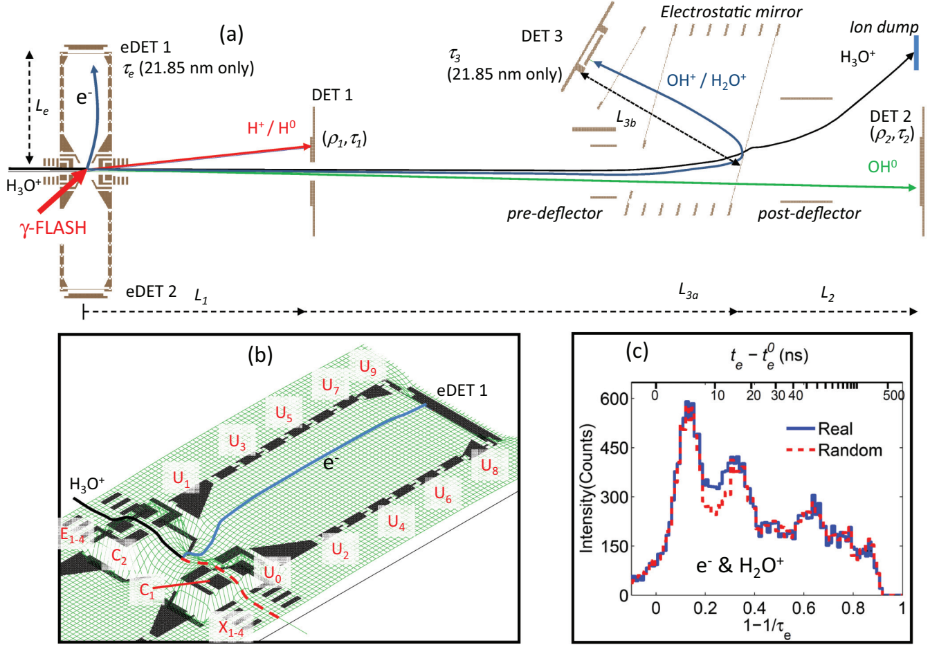
FIG. 2. (Color online) (a) Illustration of the interaction region at the TIFFF experiment [25,29] at the FLASH facility [26,27]. For the experiment at 35.56 nm, DET 3, the predeflector and the electrostatic mirror were not installed. The dashed arrows indicate the distances from the center of the interaction region to eDET 1 ( L_e = 0.142 m), to DET 1 ( L_1 = 0.263 m), to DET 2 ( L_2 = 0.872 m during measurement at 35.56 nm and L_2 = 0.967 m at 21.85 nm), as well as the horizontal distance from the interaction point to the most distant surface of the electrostatic mirror ( L_{3a} ) and upwards 150^\circ to the plane defined by the surface of DET 3 ( L_{3b} ); this yields L_3 = L_{3a} + L_{3b} = 0.975 m. Solid lines show simulated trajectories for the parent \text{H}_3\text{O}^+ ion (black line) and heavy photofragments observed in the present experiment. The trajectory of a photoelectron extracted perpendicular to the ion and photon beams is also illustrated. (b) Potential landscape of the interaction zone when configured with an electric saddle point potential to extract photoelectrons to eDET 1–2. Here, the electrode were biased to E_{1-4} = X_{1-4} = 0 , C_{1-2} = -144 V, U_0 = 112 V, U_1 = U_{2-7} = -30 V, and U_{8-9} = 0 . The fronts of eDET 1–2 were biased to 100 V. (c) Photoelectrons registered on eDET 1 in coincidence with \text{H}_2\text{O}^+ fragments registered on DET 3 from correlated and noncorrelated ion-photon crossings (real and random coincidences, respectively). The spectra were obtained at 21.85 nm with reduced laser intensity ( \sim 2.9 \mu\text{J}/\text{pulse} ).
