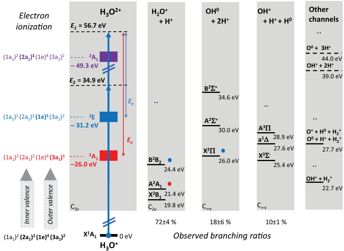
FIG. 1. (Color online) Illustration of the fragmentation channels accessible after valence shell photoionization of the hydronium ion ( \text{H}_3\text{O}^+ ) at the applied XUV energies ( E_1 and E_2 ). Calculated potential energy surfaces for the dication ( \text{H}_3\text{O}^{2+} ) electronic states in the Franck-Condon region of the ground state of \text{H}_3\text{O}^+ are not available; the energetic position of these states is estimated from the calculated orbital energies of \text{H}_3\text{O}^+ [23] and Koopmans' theorem [32]. The energies of the fragmentation limits are derived from data available at NIST [33]. The blue dot (at B^2B_2 and X^2\Pi ) and the red dot (at A^2A_1 ) mark final states identified after ionization into the {}^2E and {}^2A_1 states of \text{H}_3\text{O}^{2+} , respectively.
