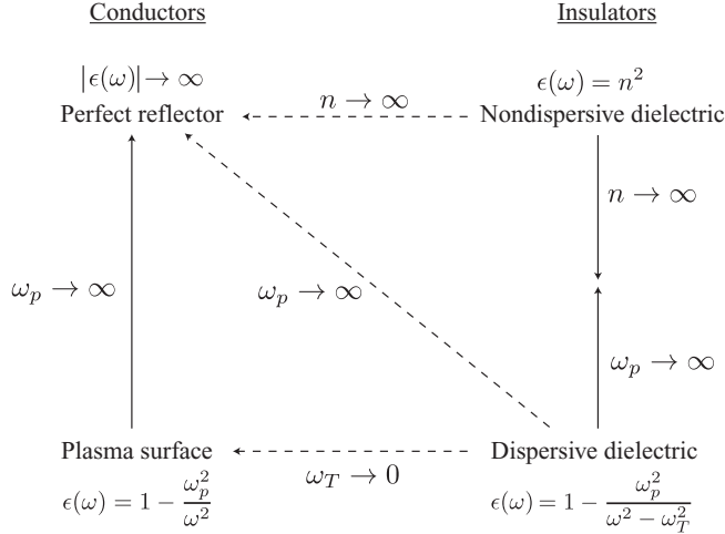
FIG. 10. Commutation properties of the various models discussed in the text. Each arrow indicates a limit which takes one dielectric function to another. Solid (dashed) arrows indicate a limit that, when applied the reflection coefficients, commutes (does not commute) with the limit k_z \rightarrow -ik_{\parallel} . The consequence of this is that the magnetic-moment results for two models connected by solid (dashed) arrows are (are not) obtainable as limiting cases of one another.
