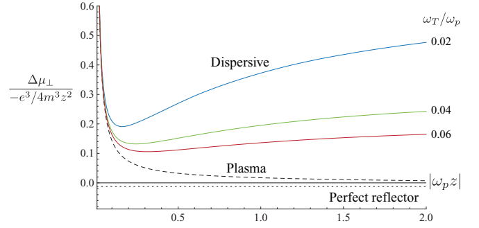
FIG. 11. (Color online) Magnetic-moment shift for dispersive dielectric and plasma models as a function of scaled distance |\omega_p z| from the surface, for the case of the magnetic field \mathbf{B}_0 perpendicular to the surface and \omega_T/\omega_p = \{0.02, 0.04, 0.06\} .
