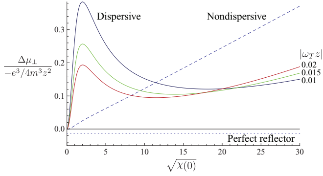
FIG. 9. (Color online) Magnetic-moment shift for dispersive and nondispersive dielectric models as a function of static susceptibility, for the case of the magnetic field \mathbf{B}_0 perpendicular to the surface and |\omega_T z| = \{0.01, 0.015, 0.02\} .
