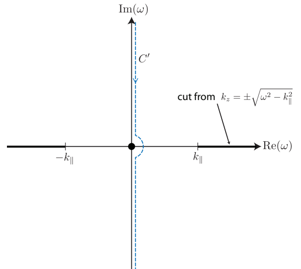
FIG. 7. (Color online) Integration path C' in the complex \omega plane.
