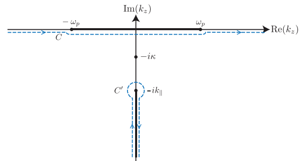
FIG. 5. (Color online) Complex k_z plane for plasma surface.
