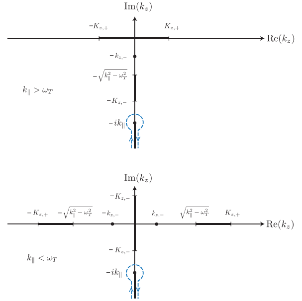
FIG. 6. (Color online) Complex k_z plane for dispersive dielectric surface.
