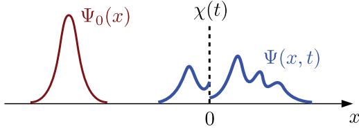
FIG. 1. (Color online) Time evolution of a quantum state in the presence of a time-dependent absorbing shutter.
