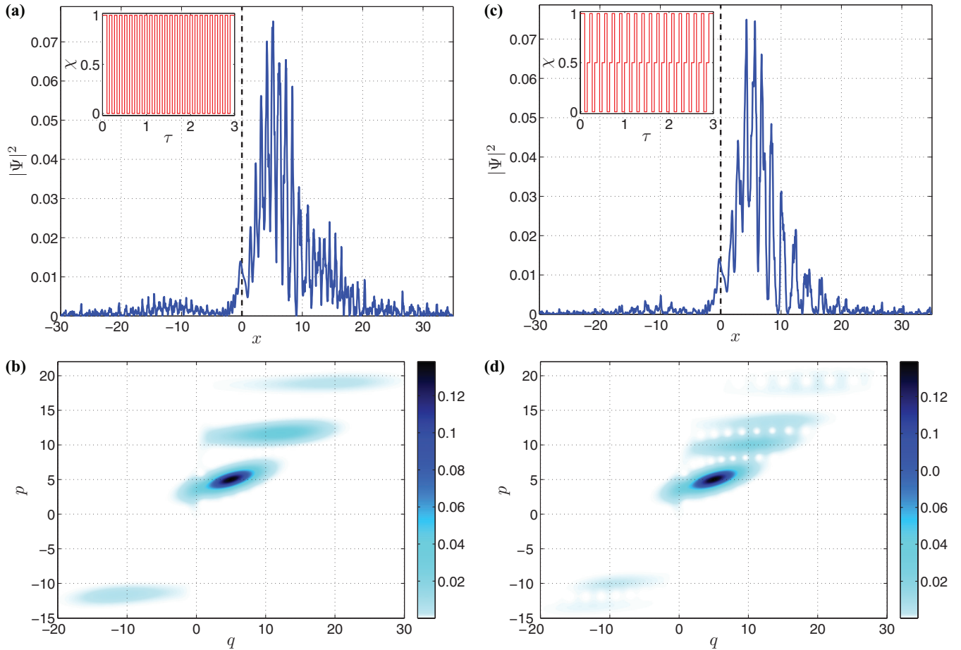
FIG. 2. (Color online) Diffraction in time of an initially Gaussian wave packet. Figures (a) and (b) show, respectively, the probability density and Husimi representation of the diffracted wave packet for the aperture function given in the inset of (a). Similarly, figures (c) and (d) correspond to the aperture function given in the inset of (c). All quantities are given in atomic units, m = \hbar = 1 .
