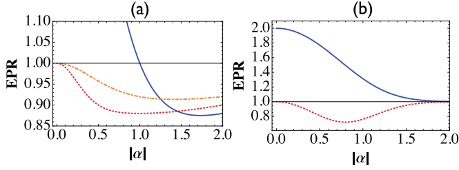
FIG. 2. (Color online) Second-order EPR correlation of the non-Gaussian entangled state (2.1) as a function of |\alpha| . (a) |\psi\rangle_A = \hat{a}^\dagger|\alpha\rangle : n+m=0 (blue solid line), 1 (red dotted line), and 2 (orange dashed line); (b) |\psi\rangle_A = |\alpha\rangle - |-\alpha\rangle : n+m = even (blue solid line) and odd (red dotted line).
