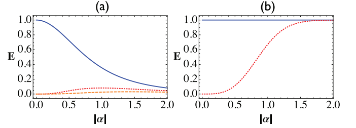
FIG. 1. (Color online) Degree of entanglement for the non-Gaussian entangled state (2.1) as a function of |\alpha| . (a) |\psi\rangle_A = \hat{a}^\dagger|\alpha\rangle : n + m = 0 (blue solid line), 1 (red dotted line), and 2 (orange dashed line); (b) |\psi\rangle_A = |\alpha\rangle - |-\alpha\rangle : n + m = \text{even} (blue solid line) and odd (red dotted line).
