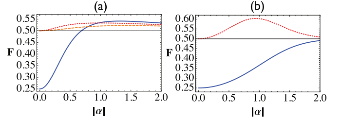
FIG. 3. (Color online) Teleportation fidelity of a coherent state with the non-Gaussian entangled resource (2.1) as a function of |\alpha| . (a) |\psi\rangle_A = \hat{a}^\dagger|\alpha\rangle : n+m=0 (blue solid line), 1 (red dotted line), and 2 (orange dashed line); (b) |\psi\rangle_A = |\alpha\rangle - |-\alpha\rangle : n+m = even (blue solid line) and odd (red dotted line).
