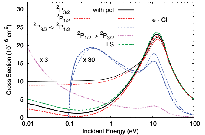
FIG. 2. (Color online) Angle-integrated cross section for elastic electron scattering from chlorine atoms in the (3p^5)2P_{3/2}^o and (3p^5)2P_{1/2}^o states, for the inelastic {}^2P_{3/2}^o \rightarrow {}^2P_{1/2}^o transition, and the superelastic {}^2P_{1/2}^o \rightarrow {}^2P_{3/2}^o transition. The latter results have been multiplied by factors of 30 and 3, respectively, for better visibility. The thick (thin) lines correspond to results obtained with (without) the polarizability effect. The curve labeled “LS” represents the nonrelativistic results for elastic scattering.
