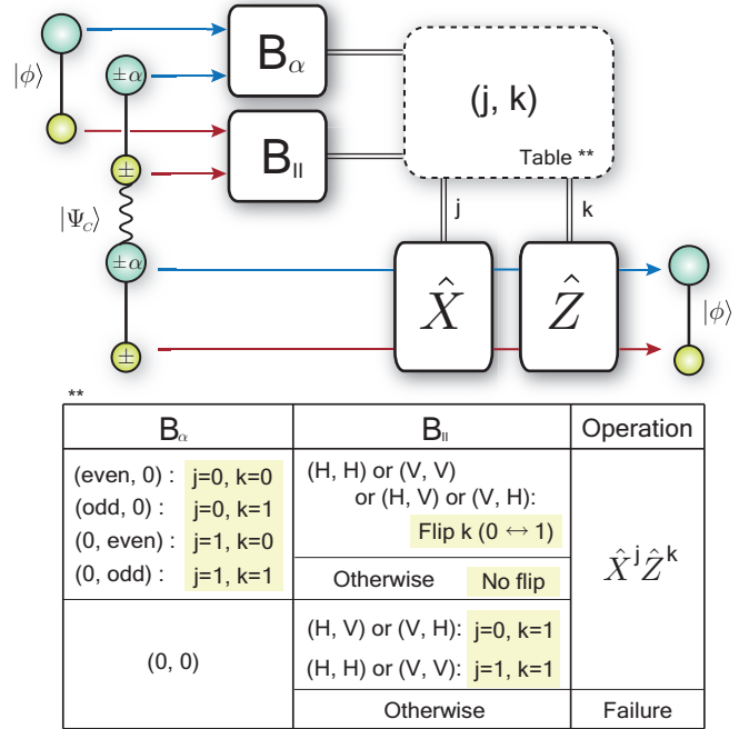
FIG. 1. (Color online) Scheme for near-deterministic quantum teleportation for a hybrid qubit using linear optics and photon detection. An unknown hybrid qubit, |\phi\rangle = a|0_L\rangle + b|1_L\rangle , is teleported through channel |\Psi_C\rangle \propto |0_L\rangle|0_L\rangle + |1_L\rangle|1_L\rangle . B_\alpha and B_{II} are performed on coherent-state modes and photon modes, respectively, between the qubit and one party of the channel state. All possible outcomes and corresponding feed-forward operations are presented in the table. A failure occurs when both B_\alpha and B_{II} fail. The failure probability is found to be P_f = \exp(-2\alpha^2)/2 . In order to perform Hadamard and CZ gates, entangled states |Z\rangle and |Z'\rangle should be used, respectively, instead of |\Psi_C\rangle .
