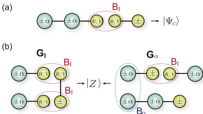
FIG. 2. (Color online) Schemes to prepare entangled channels. (a) A maximally entangled state, |\Psi_C\rangle , is generated using a B_I operation out of a two-photon pair and a hybrid pair of \sqrt{2}\alpha . In a single-photon mode, \pm and H|V denote bases \{|+\rangle, |-\rangle\} and \{|H\rangle, |V\rangle\} , respectively, which can be modified by a polarization rotation before performing the B_I operation. A 50:50 beam splitter, used to split the coherent-state part with amplitude \sqrt{2}\alpha into two modes, is omitted in the figure. (b) Two schemes, G_I and G_\alpha , to generate |Z\rangle . In G_I , two B_I operations are performed on one two-photon pair and two hybrid pairs so as to link them. The other method, G_\alpha , requires three hybrid pairs with B_I and B_\alpha operations. One of those hybrid pairs has amplitude \sqrt{2}\alpha to obtain a three-mode state |+\rangle|\alpha\rangle|\alpha\rangle + |-\rangle|-\alpha\rangle|-\alpha\rangle by a 50:50 beam splitter (omitted in the figure). Appropriate feedforwards with Pauli operations are necessary for all B_I and B_\alpha operations dependent on the measurement outcome.
