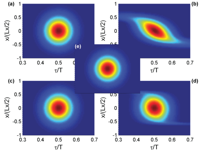
FIG. 3. (Color online) Forward retrieval fields for (a), (c) \theta_0 = \pi/2 and (b), (d) \theta_0 = \pi/9 . (e) shows the signal field to be stored. The vertical axis x/(L_x/2) is the transverse dimension of the sample normalized by the half transverse size L_x/2 ; the horizontal axis \tau/T is the local time normalized by the duration of the storage(retrieval) process T . The color indicates the signal field amplitude. (a), (b) Retrieval fields for constant \Delta\theta . The field is distorted for small \theta_0 because (1) the absolute value of \beta_z = -\beta \sin \theta_0 becomes smaller such that it approaches the lower limit of (29); and (2) \beta_x = \beta \cos \theta_0 becomes large enough to lead a spacial-temporal distortion. (c), (d) Retrieval fields for constant \Delta\theta \sin \theta_0 . There is transverse distortion of the retrieval field due to the non-vanishing \beta_x . The figures are generated under the following parameters: \lambda_s \approx \lambda_c = 1550 nm (fiber-optic communication band), |g|^2 N = 8.3 \times 10^{10}/(\text{sm}) , \Delta t/T = 1/20 , T = 1000 ns, 2R/L_x = 1/6 , where R is considered to be the transverse spatial half-width of the input signal, L_x = 0.6 cm, L = 1 cm, \Delta\theta = 8 \times 10^{-3} rad in (a) and (b), = 8 \times 10^{-3}/\sin \theta_0 rad in (c) and (d).
