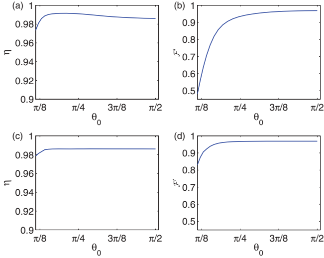
FIG. 4. (Color online) Forward retrieval efficiency \eta and fidelity \mathcal{F} vs the average polar angle \theta_0 . (a) Efficiency and (b) fidelity for forward retrieval with \Delta\theta kept as constant. (c) Efficiency and (d) fidelity for forward retrieval with \Delta\theta \sin\theta_0 kept as constant. The parameters are the same as described in Fig. 3.
