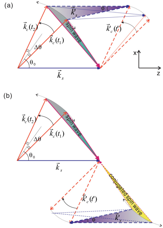
FIG. 2. (Color online) Diagram of the signal wave vector, control wave vector, and spin wave vector for (a) forward retrieval and (b) backward retrieval. A writing control wave vector changes direction from \mathbf{k}_c(t_1) to \mathbf{k}_c(t_2) . For t_1 = -T , t_2 = 0 , the control wave vector sweeps an angle 2\Delta\theta around an average polar angle \theta_0 . When a reading control field is applied at time t' , the retrieved signal field spreads over an angle \varphi . In backward retrieval, the spin waves need to be flipped to their conjugated components in the time interval between the end of the storage and the beginning of the retrieval.
