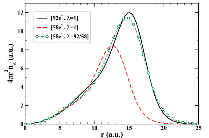
FIG. 1. (Color online) 4\pi r^2 n_\lambda versus the radial distance r for the 58e^- Na jellium cluster ( \lambda = 1 and \lambda = 92/58 ), and for the 92e^- Na jellium cluster ( \lambda = 1 ). The areas under the curves are the total number of electrons (58 and 92, respectively).
