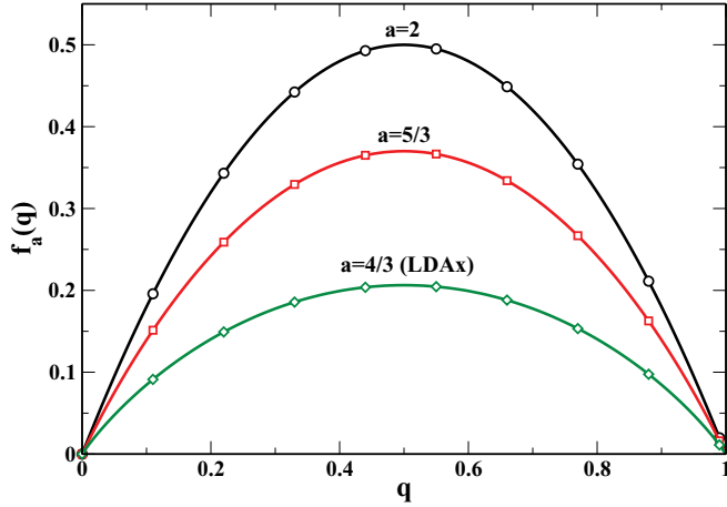
FIG. 2. (Color online) Plot of f_a(q) = 1 - q^a - (1 - q)^a for several values of the parameter a .
