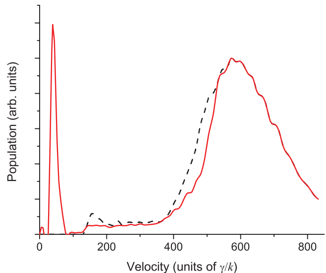
FIG. 9. (Color online) Monte Carlo modeling for the velocity distribution of a fully realized chirped BCF slower acting on a cw atomic beam, with \delta = 123\gamma and a 600-MHz chirp with a ramp duration of 10 \mu s. The black dashed line is the velocity distribution of the atomic beam source, and the red solid line is the predicted distribution with the chirped BCF present. Notice the large slow atom peak at \sim 50\gamma/k and the relatively uniform depletion of a large range of atomic velocities.
