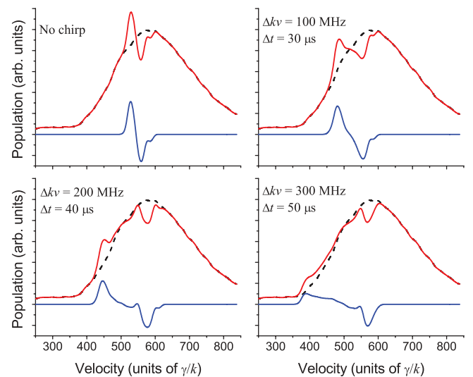
FIG. 8. (Color online) Chirped BCF Monte Carlo model output after reducing BCF magnitude, using the same experimental parameters used to obtain the results in Fig. 7.
