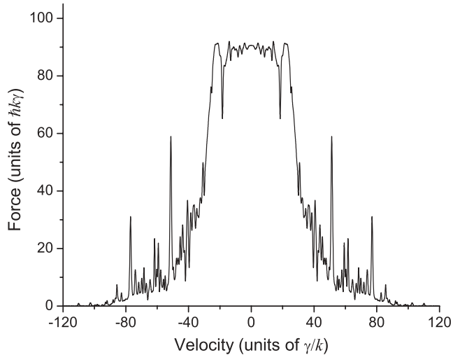
FIG. 2. Calculated bichromatic force vs velocity for \delta = 154\gamma and phase \phi = \pi/2 , for \Omega_{\text{opt}} = \sqrt{3/2}\delta . This optimum Rabi frequency yields the largest central force, in agreement with Eq. (5) rather than Eq. (1). Note that the force magnitude is shown as a multiple of \hbar k\gamma , which is twice the radiative force F_{\text{rad}} .
