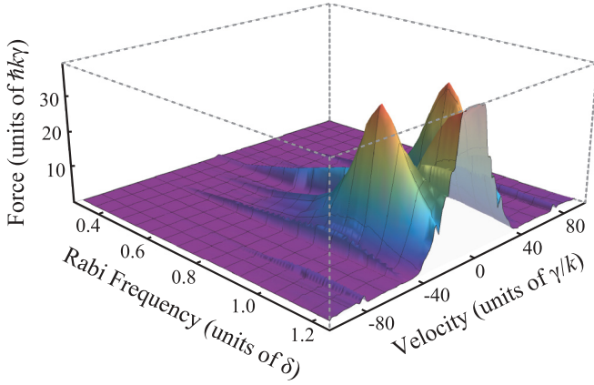
FIG. 5. (Color online) Three-dimensional BCF surface used in the Monte Carlo chirped BCF models. The beat-note phase is assumed constant over the interaction region so that the force is a function only of the atomic velocity and Rabi frequency. The surface is interpolated from numerical solutions to the OBEs. The force is zero at Rabi frequencies less than 0.4\delta and absolute velocities greater than 100\gamma/k .
