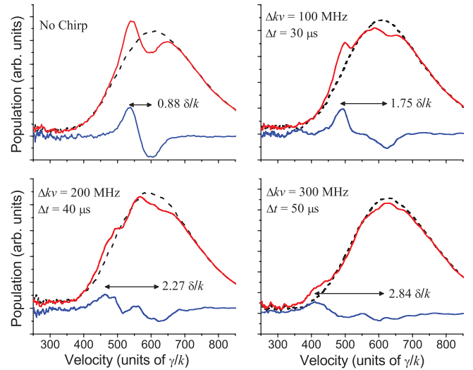
FIG. 7. (Color online) Experimentally observed velocity profiles for frequency-chirped BCF slowing with \delta = 74\gamma , \Omega_r = \sqrt{3/2}\delta , and \phi = \pi/2 . The four panels show chirp ramps of 0 MHz, 100 MHz in 30 \mu\text{s} , 200 MHz in 40 \mu\text{s} , and 300 MHz in 50 \mu\text{s} .
