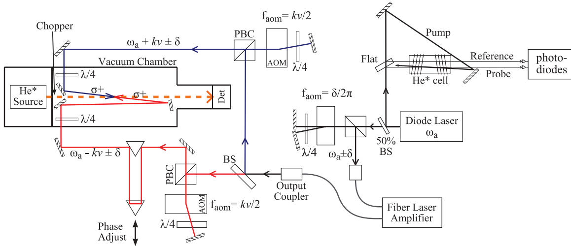
FIG. 3. (Color online) Experimental configuration for observing the BCF in atomic He using detunings of 123\gamma – 278\gamma with a static Doppler shift centered at atomic velocity v . Polarizing beam-splitter cubes are denoted by PBC, and a beam splitter by BS.
