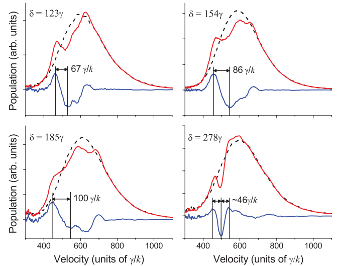
FIG. 4. (Color online) Experimentally observed velocity profiles for BCF slowing, increasing in detuning from top to bottom. The dotted trace (black) is the unsloped distribution, the upper solid trace (red) is the slowed distribution, and the lower solid trace (blue) is the difference. Notice the anomalous result at \delta = 278\gamma , consistent with previous observations of an upper limit to the BCF detuning.
