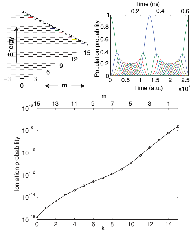
FIG. 2. (Color online) Upper left panel: Stark states |km\rangle of the n = 16 level due to the constant electric field \epsilon_z . Only the states with m \geq 0 are shown. The states populated by the rotating microwave field in the xy plane are shown in color and with arrows. Upper right panel: The population of the (colored) Stark states as a function of time for one round trip in the Stark setup, corresponding to time \tau = 2.61 \times 10^7 a.u. The initial state is the circular Stark state. After half the cycle \tau the most polarized state is fully populated while the circular state is depleted. At the end of the round trip the circular state is totally revived. Lower panel: The ionization probability of the relevant Stark |km\rangle states when fully populated. Field parameters are given in the text.
