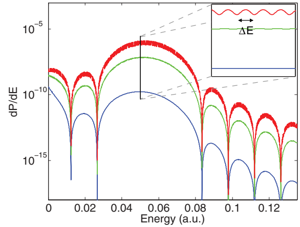
FIG. 4. (Color online) Energy distribution of the continuum wave packet for a series of pulses, N = 3 (lower, blue line), 4 (middle, green line), and 5 (upper, red line). The time separation between the pulses is \Delta t = 3 \times 10^6 a.u. Succeeding pulses hitting states with ionization probability differing only a few orders in magnitude cause interference in the continuum wave packet as observed between the fourth and the fifth pulse (upper line). The inset shows a closeup of the distributions on the interval (0.05, 0.05 + 10^{-5}) a.u. The period of the oscillations clearly matches the time delay between the pulses, i.e., \Delta E = 2\pi/\Delta t \simeq 2.1 \times 10^{-6} a.u. Field parameters are given in the text.
