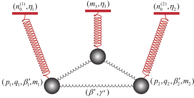
FIG. 1. (Color online) A schematic illustration for the three coupled nonrigid pendulums, with three pairs of canonical variables: (n_0^{(1)}, \eta_1) , (n_0^{(2)}, \eta_2) , and (m_3 = m_1 - m_2, \eta_3) . The first two pairs describe intraspecies spin mixing dynamics, while the remaining third pair denotes interspecies spin mixing dynamics.
