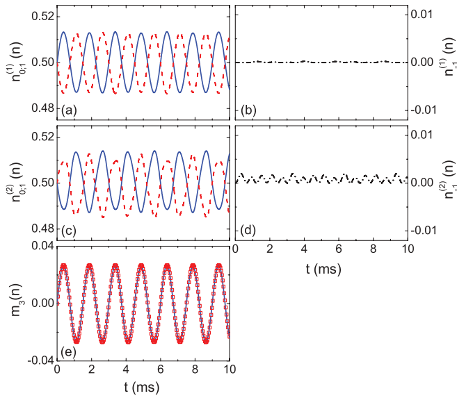
FIG. 3. (Color online) Population dynamics for all spin components, with the interspecies interaction parameters \beta' = 5|\beta'_1| and \gamma' = 2|\beta'_1| and the quadratic Zeeman shifts q_1 = 30|\beta'_1|n and q_2 = q_1\Delta E_2/\Delta E_1 . (a) For ^{87}\text{Rb} atoms, the blue solid line and red dashed line represent the M_F = 1, 0 components, respectively. (b) As in panel (a), but the M_F = -1 component is represented by the black dotted dash line. (c) and (d) As in panels (a) and (b), respectively, but for ^{23}\text{Na} atoms. (e) Time evolution of m_3 . The blue solid line and the red square symbols denote numerical and analytical solutions, respectively.
