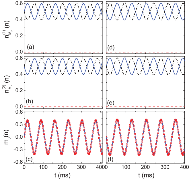
FIG. 2. (Color online) Population dynamics for every spin component. For panels (a)–(c), the interspecies interaction parameters used are \beta' = 5|\beta'_1| and \gamma' = 2|\beta'_1| . For panels of (d)–(f), \beta' = 5|\beta'_1| and \gamma' = -2|\beta'_1| are used. (a) For ^{87}\text{Rb} atoms, the blue solid line, the red dashed line, and the black dotted-dash line represent the M_F = 1 , 0, and -1 components, respectively. (b) As in panel (a), but for ^{23}\text{Na} atoms. (c) Time-dependent m_3 . The blue solid line and the red square symbols denote numerical and analytical solutions, respectively. (d) As in panel (a), but with \gamma' = -2|\beta'_1| . (e) As in panel (b), but with \gamma' = -2|\beta'_1| . (f) As in panel (c), but with \gamma' = -2|\beta'_1| .
