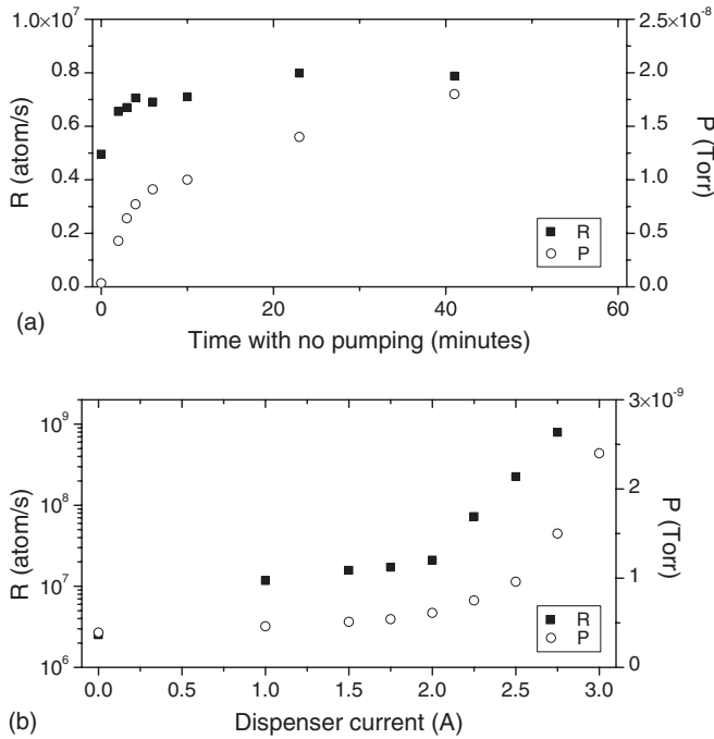
FIG. 2. Response of the pressure gauge reading P and the MOT loading rate R to (a) turning off the chamber pumps and (b) increasing the Rb dispenser current.
