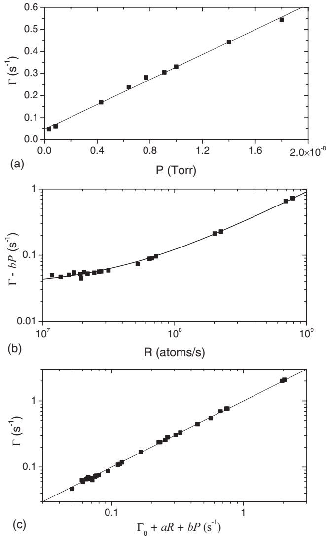
FIG. 3. Dependence of the MOT loss rate \Gamma on the load rate R and gauge pressure P . (a) Response to turning off the chamber pumps as in Fig. 2(a). The line is a linear fit. (b) Response to increasing the dispenser current as in Fig. 2(b). The curve is a linear fit. (c) Comparison between the measured loss rate \Gamma and the model loss rate \Gamma_{\text{fit}} = \Gamma_0 + aR + bP , for fit parameters \Gamma_0 = 0.036 \text{ s}^{-1} , a = 8.55 \times 10^{-10} , and b = 2.9 \times 10^7 \text{ Torr}^{-1} \text{ s}^{-1} . The line shows \Gamma = \Gamma_{\text{fit}} .
