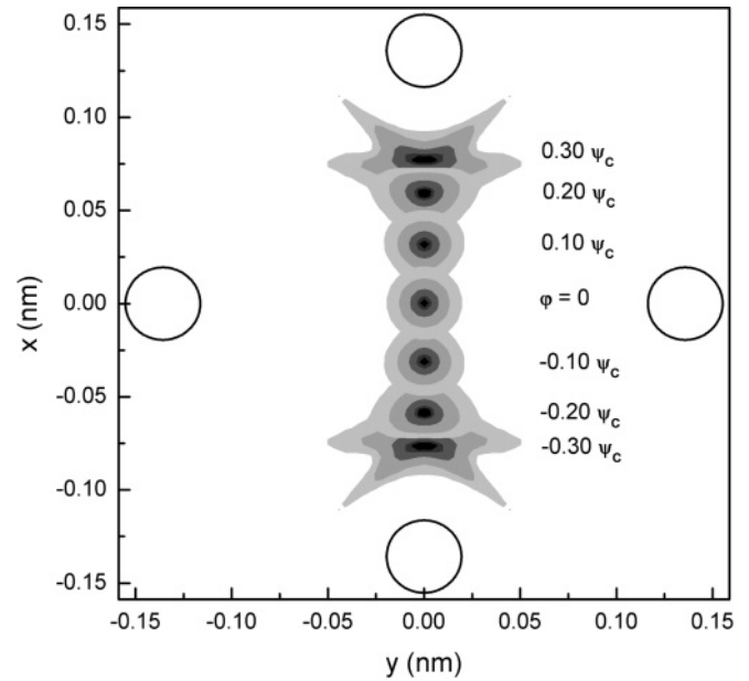
FIG. 3. The yields of channeled protons in the transverse position plane in the two-dimensional representation for the proton beam incident angles \varphi = 0 , \pm 0.10\psi_c , \pm 0.20\psi_c , and \pm 0.30\psi_c and the reduced crystal thickness \Lambda = 0.250 , corresponding to the crystal thickness L = 481.8 nm, with the effects of the crystal's electrons taken into account. The area in which the yield of channeled protons is below 5 % is designated by white color, the areas in which the yields are between 5 and 10 %, 10 and 15 %, 15 and 20 %, 20 and 50 %, and 50 and 80 % by the increasing tones of gray color, respectively, and the area in which the yield is above 80 % by black color. The atomic strings defining the channel are represented by the circles lying on the x and y axes.
