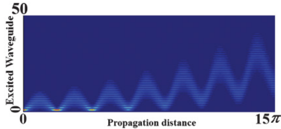
FIG. 3. (Color online) Theoretical evolution of the probability of having one photon at waveguide n when launched at channel 0, P_{n,0}(Z) = \langle a_n^\dagger a_n \rangle , under the resonance condition.
