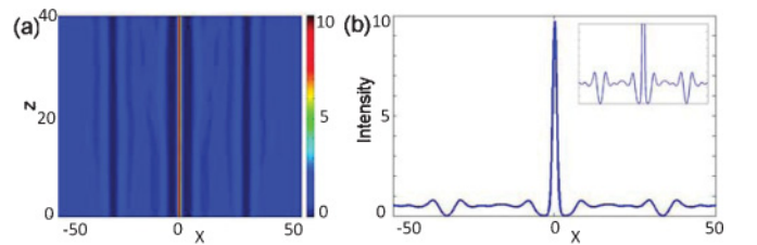
FIG. 10. (Color online) Coexistence of bright and dark solitons in media with competing nonlinearities. (a) Dynamics of soliton propagation. (b) Intensity profile of bright and dark solitons located on the same constant background. (Inset) Details of the dark solitons. The solitons have been excited using the following initial conditions: u(x, 0) = 1.911 \exp[-(x/20.97)^2] - 0.72 \tanh[(0.66(x - 30))] \tanh[(0.66(x + 30))] . The medium parameters are \alpha_1 = 1 , \alpha_2 = -2 , \sigma_1 = 1 , and \sigma_2 = 3 .
