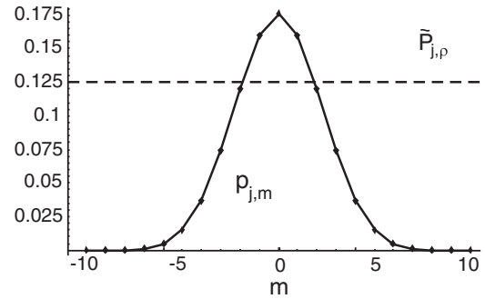
FIG. 1. Plot of p_{j,m} (diamonds joined by a solid line) and \tilde{\mathcal{P}}_{j,\rho} (dashed line) for a phase-averaged SU(2) coherent state with j = 10 showing that the classical bound is clearly infringed by the statistics of the outcomes m = 0, \pm 1 .
