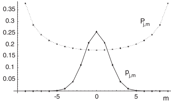
FIG. 4. Plot of the statistics of j_{\perp,1} (diamonds joined by solid line) for the state (3.24) for j = 10 , \eta = 0.5 along with the SU(2) classical state upper bound (3.5) (stars joined by dotted line) showing the violation of the classical bounds for small |m| .
