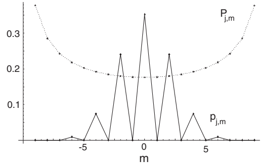
FIG. 3. Plot of the j_1 statistics p_{j,m} (diamonds joined by solid line) for the Schrödinger cat state (3.21) and the SU(2) bound for classical states \mathcal{P}_{j,m} (stars joined by a dotted line) in Eq. (3.5) for j = 10 showing that for m = 0, \pm 2 there is a clear violation of the classical upper bound.
