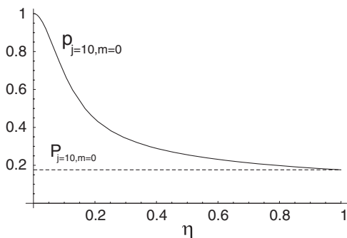
FIG. 5. Plot of the probability p_{j, m=0} (solid line) of the eigenvalue m = 0 of j_{\perp,1} for the state (3.24) with j = 10 as a function of \eta along with the SU(2) classical upper bound (3.6) \mathcal{P}_{j, m=0} (dashed line) showing nonclassical behavior for all \eta < 1 .
