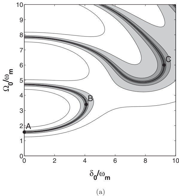
FIG. 5. (a) Magnified map of P_{\text{nad}} for sinusoidal pulses. The curves are for P_{\text{nad}} = 0.1, 0.01, 0.001, \dots . Point A is the \pi pulse, and points B and C are the adiabatic pulses. (b) P_{\text{nad}} with Doppler shift for the points A, B, and C.
