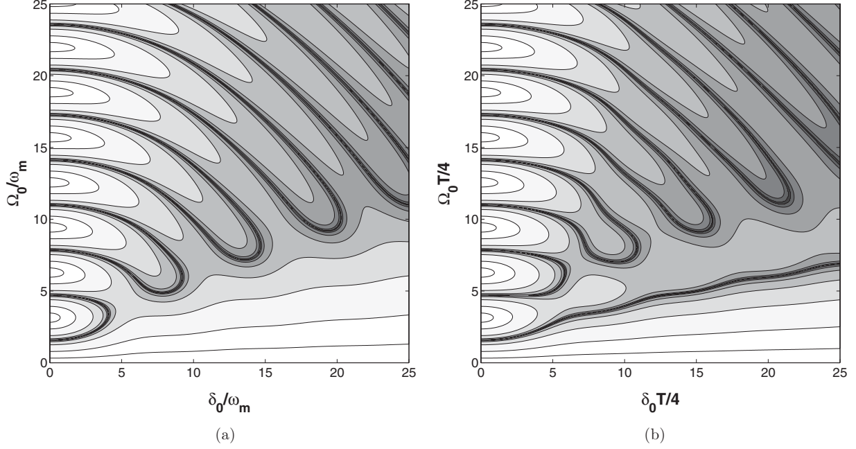
FIG. 1. Map of P_{\text{nad}} in the pulse parameter space. The curves are for P_{\text{nad}} = 0.9, 0.5, 0.1, 0.01, 0.001, \dots . The darkest regions are for vanishing P_{\text{nad}} . (a) Sinusoidal pulse. (b) Triangular pulse.
