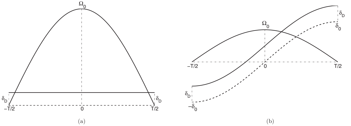
FIG. 4. Profiles of Doppler-shifted pulses. Dashed lines are the detuning without Doppler shift. (a) \pi pulse. (b) Adiabatic pulse.
