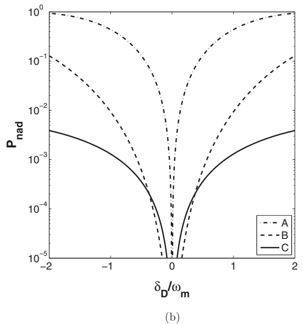
FIG. 5. (a) Magnified map of P_{\text{nad}} for sinusoidal pulses. The curves are for P_{\text{nad}} = 0.1, 0.01, 0.001, \dots . Point A is the \pi pulse, and points B and C are the adiabatic pulses. (b) P_{\text{nad}} with Doppler shift for the points A, B, and C.
