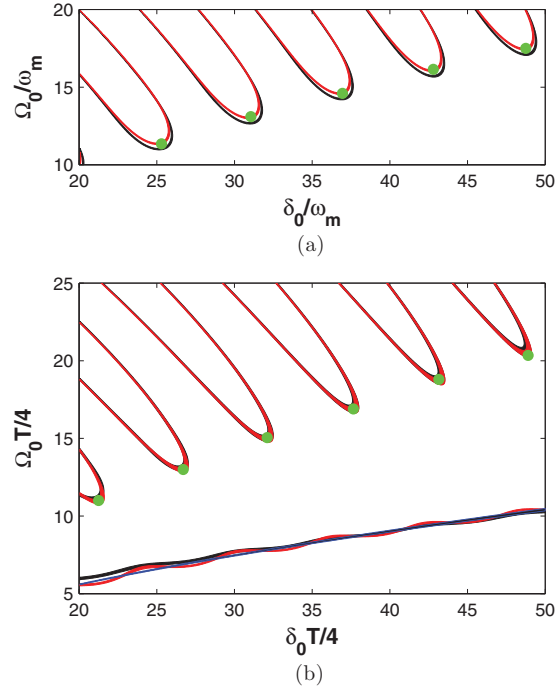
FIG. 3. (Color online) Trace of P_{\text{nad}} = 0 in the map along the boundary between the oscillatory and nonoscillatory regions. (a) Sinusoidal pulse. Black curves, exact P_{\text{nad}} ; red (gray) curves, approximate P_{\text{nad}} given by Eq. (3.2); and dots, tips of loops given by Eq. (3.3). (b) Triangular pulse. Black curves, exact P_{\text{nad}} ; red (gray) curves, approximate P_{\text{nad}} given by Eq. (3.1); lower blue (thin) curve, approximate P_{\text{nad}} given by Eq. (3.4); and dots, tips of loops given by Eq. (3.5).
