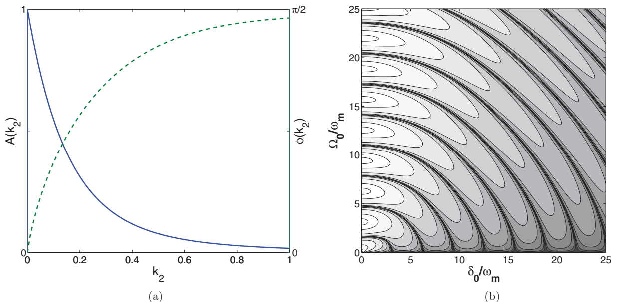
FIG. 2. (Color online) (a) Amplitude (solid line) and phase factor (dashed line) of P_{\text{nad}} in Eq. (2.2). (b) Map of P_{\text{nad}} in Eq. (2.2) for sinusoidal pulses. The curves are for P_{\text{nad}} = 0.9, 0.5, 0.1, 0.01, 0.001, \dots
