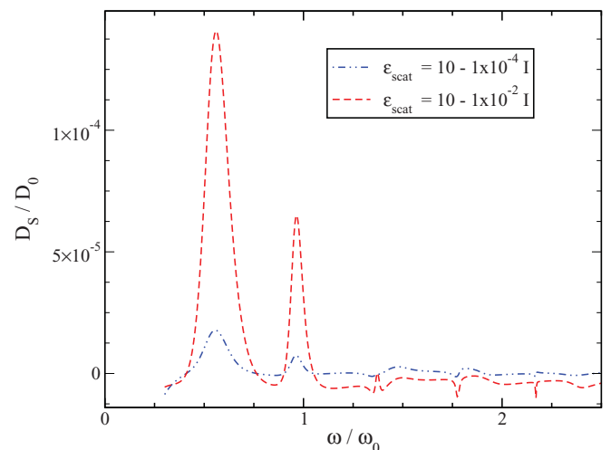
FIG. 3. (Color online) Normalized extra contribution to the diffusion coefficient D_s/D_0 for different values of the optical gain as a function of the dimensionless frequency.
