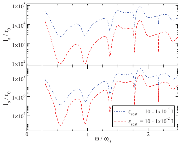
FIG. 7. (Color online) Displayed in the upper panel is the two-particle amplification length \ell_a for different values of the optical gain as a function of the dimensionless frequency. Displayed in the lower panel is the two-particle oscillation length \ell_o for different values of the optical gain as a function of the dimensionless frequency.
