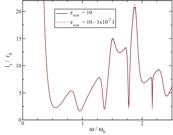
FIG. 6. (Color online) Displayed here is the single-particle scattering mean-free path l_s for amplifying scatterers and conserving scatterers. The difference between the two is seen to be small and mainly manifests itself in narrow dips and peaks.
