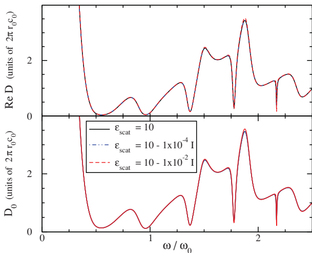
FIG. 5. (Color online) Real part of diffusion coefficient D(0) (upper panel) and the bare diffusion coefficient D_0 (lower panel) for different values of the optical gain as a function of the dimensionless frequency. The diffusion coefficients are shown in natural units ( 2\pi r_0 c ), r_0 is the scatterer's radius, and c is the vacuum speed of light. The influence of optical gain on diffusion is seen to be small.
