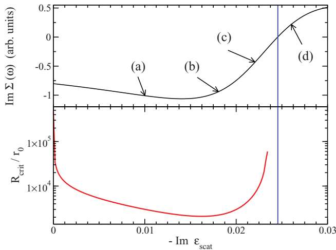
FIG. 10. (Color online) The upper panel shows the imaginary part of the self-energy at a fixed frequency ( \omega/\omega_0 \simeq 2.1710269 ) as a function of gain; cf. Fig. 9. The vertical line signalizes the zero of \text{Im}\Sigma . From Fig. 9 and the text below, it is clear that this zero indicates that the laser threshold has already been crossed. The points (a) through (d) correspond to -\text{Im}\epsilon_{\text{scat}} = \{0.01, 0.018, 0.022, 0.026\} , i.e., to the curves shown in Fig. 9. The intersections with the vertical line there yield the values shown here. The lower panel displays the critical length R_{\text{crit}} as a function of gain. Due to the off-resonant frequency, R_{\text{crit}} has a local minimum and increases again with increasing gain.
