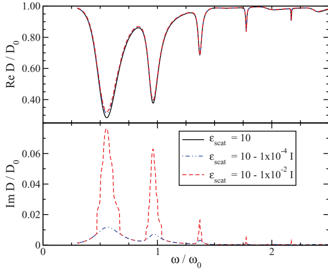
FIG. 4. (Color online) Normalized real part (upper panel) and imaginary part (lower panel) of the diffusion coefficient D(\Omega = 0) for different values of optical gain as indicated as a function of the dimensionless frequency. For the displayed frequency range, the gain value is below threshold.
