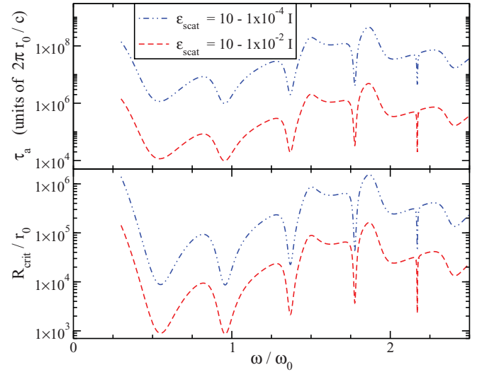
FIG. 8. (Color online) Displayed in the upper panel is the two-particle amplification time \tau_a for different values of the optical gain as a function of the dimensionless frequency. In the lower panel we show the critical length R_{\text{crit}} , characterizing the threshold volume in which the intensity experiences a laser-like growth behavior.
