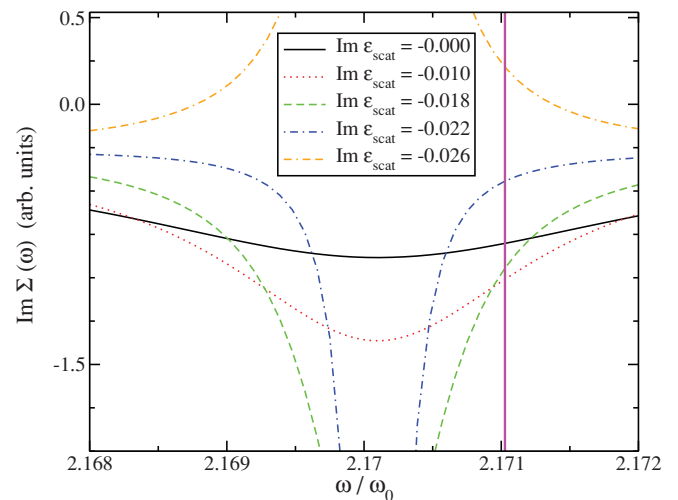
FIG. 9. (Color online) The imaginary part of the self-energy in the vicinity of the fifth Mie resonance for different but fixed values of gain. Increasing gain clearly yields narrowing and deepening until the laser threshold is reached; the curve approaches the shape of a delta function. Beyond this point the theory is not valid anymore due to physical reasons. For completeness we also show the last curve \text{Im}\epsilon_s = -0.0026 representing a system which has obviously crossed the threshold. The vertical line marks the frequency discussed in Fig. 10; see also text below.
