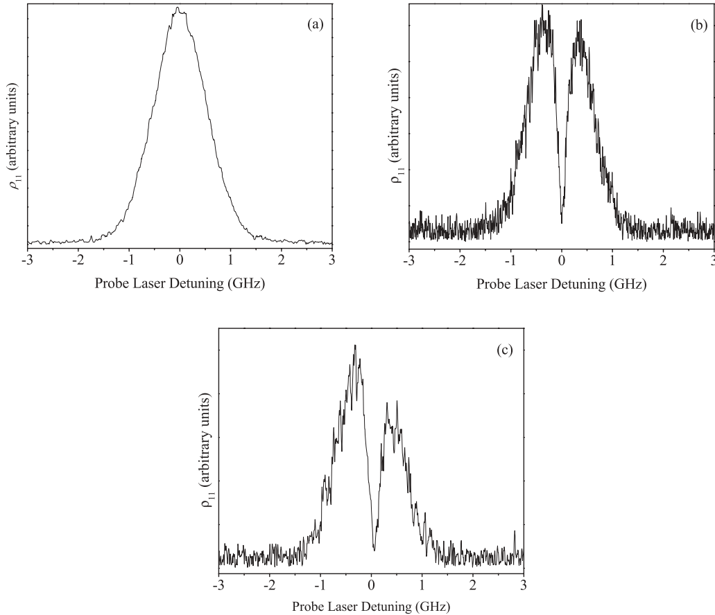
FIG. 3. Experimental spectra for \text{Na}_2 V-system probe laser scans in the copropagating geometry (a) with the coupling field turned off and (b) with the coupling field on and the frequency of the coupling laser set to line center of the transition. (c) The coupling field is detuned by \sim 60 MHz. The coupling laser power is 265–270 mW and the probe laser power is less than 1 mW.
