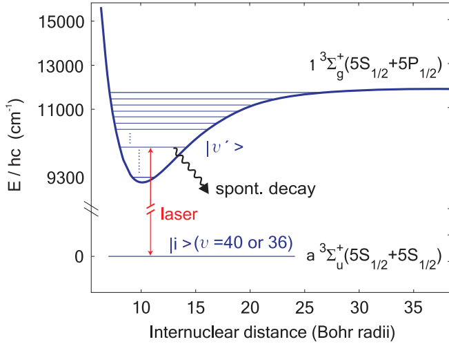
FIG. 1. (Color online) Spectroscopy scheme. A tunable laser couples the Feshbach molecule level |i\rangle to an excited level |v'\rangle with energy E in the (1)^3\Sigma_g^+ state. The excited state quickly decays spontaneously. Level positions in the (1)^3\Sigma_g^+ potential are detected through resonantly enhanced loss of Feshbach molecules; h is Planck's constant and c is the speed of light.
