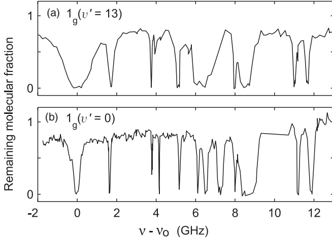
FIG. 4. The 1_g spectra of two different vibrational levels at 986.8 G. For each spectrum, we subtract a frequency offset \nu_0 from the excitation frequency \nu such that the most deeply bound line is situated at 0 GHz. (a) v' = 13 , \nu_0 = 294626.4 GHz. (b) v' = 0 , \nu_0 = 281068.2 GHz. In these two scans, not all lines that we eventually observed are resolved.
