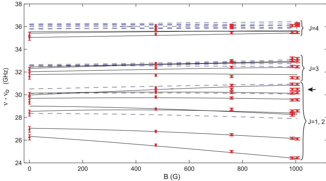
FIG. 7. (Color online) Zeeman diagram of the 1_g ( v' = 13 ) state. An offset \nu_o = 294\,600 GHz is subtracted from the excitation frequency \nu . The lines are calculations. Dashed lines indicate levels with F > 3 that cannot be observed in our experiment at B = 0 due to the selection rule F = 0, \pm 1 . The arrow points to an experimentally observed line that is not well described by the calculations. Table II gives the corresponding quantum numbers at 0 G.
