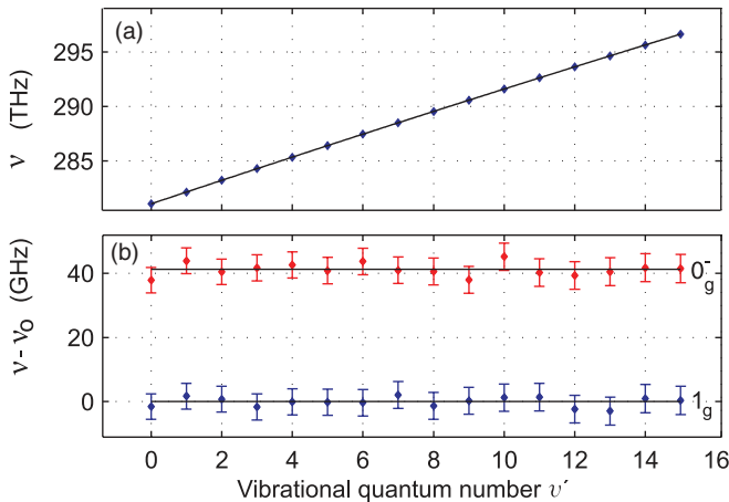
FIG. 3. (Color online) Vibrational ladder for the (1)^3\Sigma_g^+ state. (a) Excitation frequencies \nu of the vibrational states with quantum number v' . The solid line is a quadratic fit to the data. (b) Zoom into the vibrational levels, which are split into 0_g^- and 1_g components. The spectra are measured at low resolution and high power. A frequency offset \nu_o(v') is subtracted from the excitation frequency \nu for each data point. The offset \nu_o(v') is a quadratic fit to the 1_g data. Note the different energy scales of panels (a) and (b).
