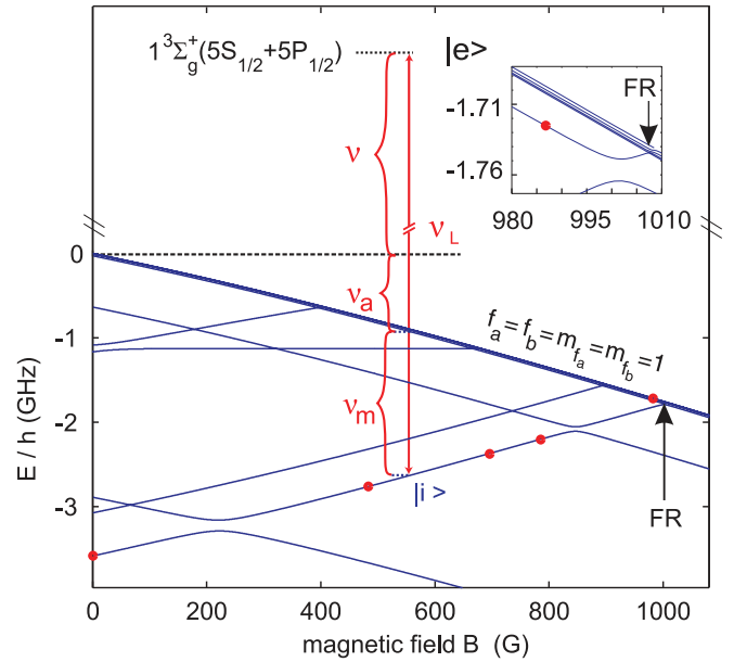
FIG. 2. (Color online) Energy diagram of the Zeeman structure for some weakly bound \text{Rb}_2 molecular states below the |f_a = 1, m_{f_a} = 1\rangle + |f_b = 1, m_{f_b} = 1\rangle atomic asymptote. Dots mark the levels and magnetic fields used for the spectroscopy. For simplicity, throughout the paper we report excitation frequencies \nu with respect to the two-atom threshold at 0 G. These are obtained by subtracting the known atomic Zeeman shift \nu_a and the known molecular binding frequency \nu_m from the excitation frequency \nu_L . The inset zooms into the region near the Feshbach resonance at 1007.4 G, marked with an arrow and "FR."
