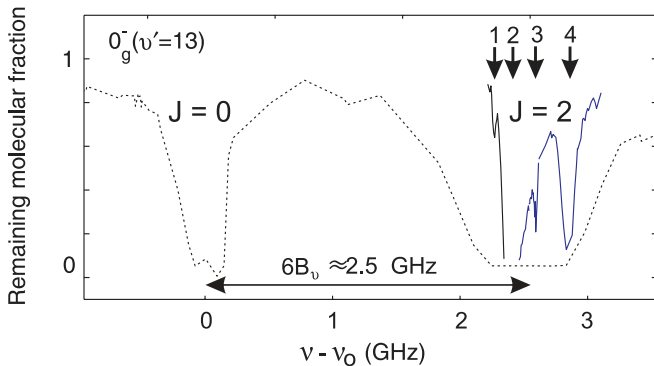
FIG. 5. (Color online) Scans of 0_g^- ( v' = 13 ) lines in the (1)^3\Sigma_g^+ state at a magnetic field of 986.8 G. The dotted line corresponds to a laser power of 0.1 mW and a pulse duration of 200 ms while the solid line corresponds to a laser power of 0.1 mW and a 1-ms pulse duration. The frequency offset is \nu_0 = 294671.0 GHz. The line at \nu - \nu_0 = 0 GHz corresponds to J = 0 , while the four lines located around 2.5 GHz have J = 2 . Due to saturation, these four lines are not resolved for the 200-ms pulse.
