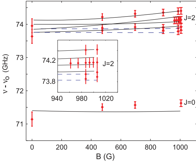
FIG. 6. (Color online) Zeeman diagram of the 0_g^-(v=13) state. An offset \nu_0 = 294\,600 GHz is subtracted from the excitation frequency \nu . The lines are calculations. Dashed lines indicate levels with F > 3 that cannot be excited in our experiment at B = 0 due to the selection rule on \Delta F = 0, \pm 1 . Table I gives the quantum numbers at 0 G and 1005.8 G. The inset is a zoom into the closely spaced lines around 1000 G.
