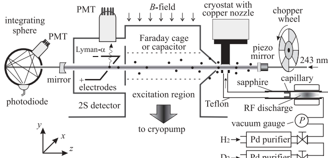
FIG. 1. Schematic of the excitation region. For the characterization of the dc Stark shift, the Faraday cage is replaced by a plane capacitor with the electric field oriented along one of the three axes (see also Fig. 3). PMT denotes a photomultiplier tube.
