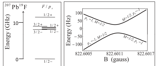
FIG. 1. Left hand side: Hyperfine energy level structure of the ground electronic ( X_1 ) and rotational ( J = 1/2 ) state of the 207 Pb 19 F molecule as a function of F (total angular momentum) and p_s (parity). Two closely spaced F = 1/2 states of opposite parity are shown by thick lines. Right hand side: Anapole-induced avoided crossing of the M_F = 1/2 sublevels of the closely spaced M_F = 1/2 states. This crossing is predicted to occur at a field of 823 \pm 40 G.
