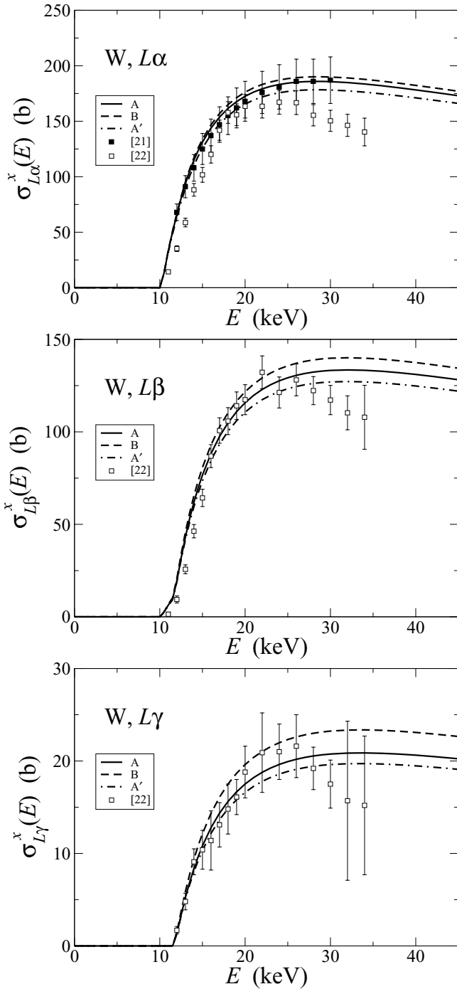
FIG. 3. X-ray production cross sections \sigma_{L\alpha}^x , \sigma_{L\beta}^x , and \sigma_{L\gamma}^x of W as a function of energy. The continuous, dashed, and dot-dashed curves correspond to the theoretical cross sections calculated with sets A, B, and A', respectively. Symbols are experimental data from Refs. [21,22].
