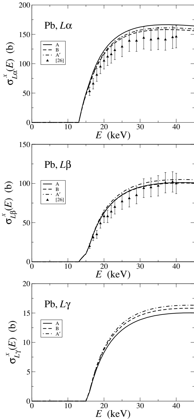
FIG. 7. X-ray production cross sections \sigma_{L\alpha}^x , \sigma_{L\beta}^x , and \sigma_{L\gamma}^x of Pb as a function of energy. The continuous, dashed, and dot-dashed curves correspond to the theoretical cross sections calculated with sets A, B, and A', respectively. Symbols are experimental data from Ref. [26].
