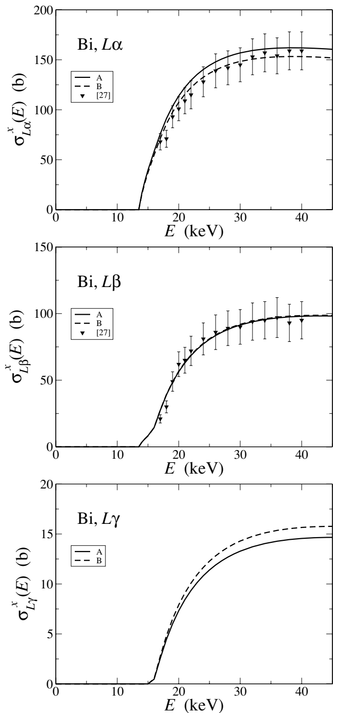
FIG. 8. X-ray production cross sections \sigma_{L\alpha}^x , \sigma_{L\beta}^x , and \sigma_{L\gamma}^x of Bi as a function of energy. The continuous and dashed curves correspond to the theoretical cross sections calculated with sets A and B, respectively. Symbols are experimental data from Ref. [27].
