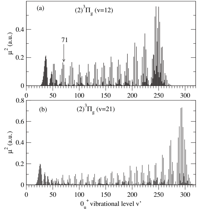
FIG. 4. Squared matrix element \mu^2 = |\langle 0_u^+, v' | D_{(2)-b} | (2)^3\Pi_g, v \rangle|^2 (in atomic units) of the transition dipole moment function D_{b-(2)} [see Fig. 1(d)]. The level v' = 71 discussed in the text is indicated for clarity. (a) v = 12 ; (b) v = 21 .
