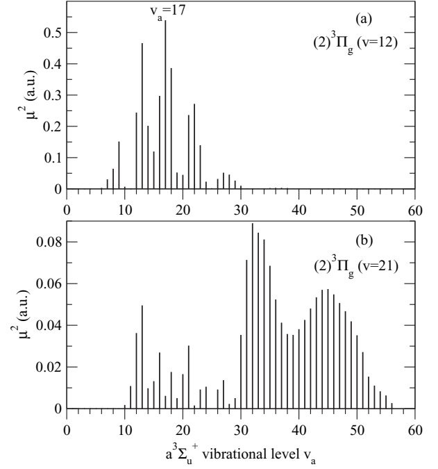
FIG. 6. Squared matrix element \mu^2 = |\langle (2)^3\Pi_g, v | D_{(2)-a} | a^3\Sigma_u^+, v_a \rangle|^2 (in atomic units) of the transition dipole moment function D_{a-(2)} [see Fig. 1(d)]. (a) v = 12 ; (b) v = 21 .
