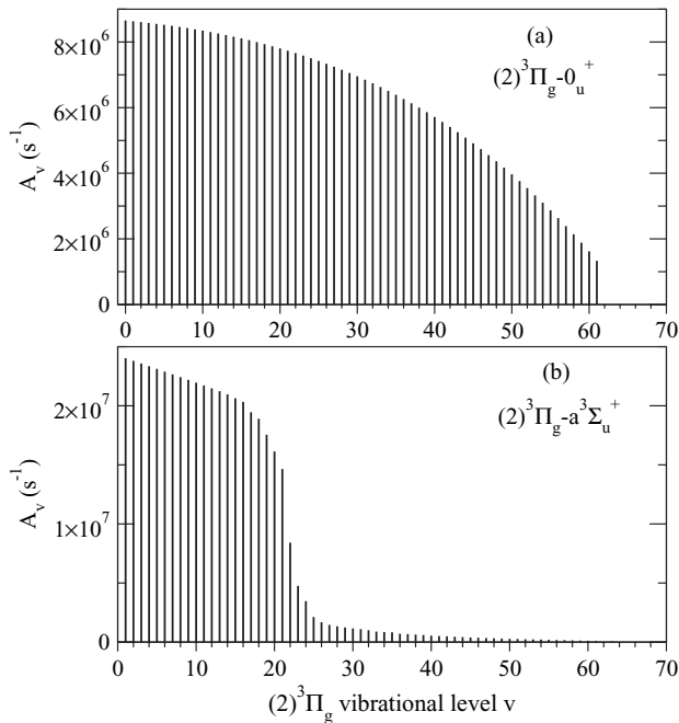
FIG. 3. Relaxation rate A_v (in s^{-1} ) of the 2^3\Pi_g vibrational levels (a) toward the levels of 0_u^+(A-b) system, and (b) toward the levels of the a^3\Sigma_u^+ state.
