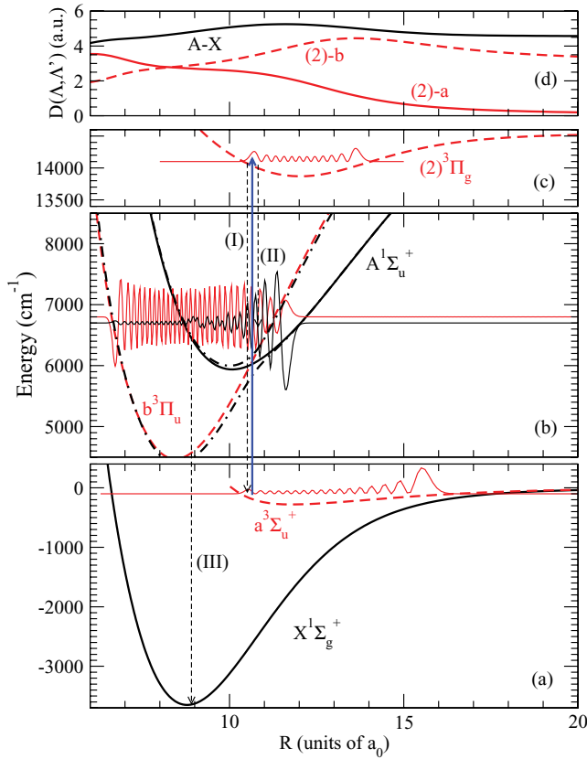
FIG. 1. (Color online) Scheme of the proposed process. (a) The a^3\Sigma_u^+ v = 17 level is initially populated by PA. (b) The A^1\Sigma_u^+(6s + 6p) and b^3\Pi_u(6s + 6p) potential curves, and the resulting 0_u^+ curves (dot-dashed lines) after diagonalization of the potential matrix of the A and b curves coupled by the spin-orbit coupling function of Ref. [33]. The (2)^3\Pi_g level can decay either directly to the a state (arrow I), or to the X state via the 0_u^+ states (arrows II and III). Probability densities are reported with an arbitrary scale. For the 0_u^+ coupled wave function, the component on the b state (upper red trace) and on the A state (lower black trace) of the wave function are both represented on the same scale. (c) It can be efficiently excited (thick vertical arrow) to the (2)^3\Pi_g v = 12 level. (d) R -dependent dipole moment for the transitions a^3\Sigma_u^+ - (2)^3\Pi_g ( D_{(2)-a} ), b^3\Pi_u - (2)^3\Pi_g ( D_{(2)-b} ), and X^1\Sigma_g^+ - A^1\Sigma_u^+ ( D_{A-X} ).
