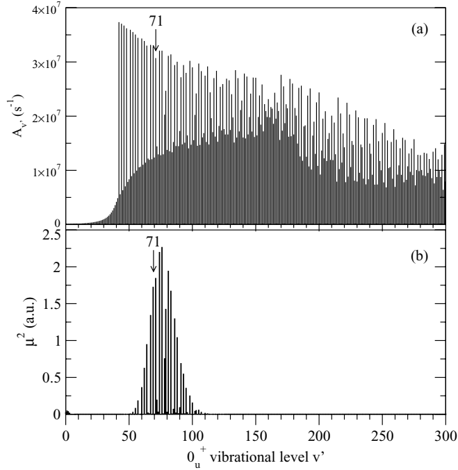
FIG. 5. (a) Relaxation rates A_{v'} (in s^{-1} ) of the vibrational levels of the 0_u^+ coupled states toward the levels of the X ground state. The v' = 71 level is indicated for clarity. (b) The squared matrix element |\langle X^1\Sigma_g^+ v'' = 0 | D_{A-X} | 0_u^+, v' \rangle|^2 , indicating that the v' = 71 0_u^+ level indeed decays efficiently to v'' = 0 .
