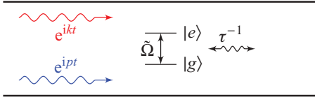
FIG. 1. (Color online) Schematic representation of two photons in a waveguide at frequencies k and p moving to the right toward a two-level atom with energy levels |g\rangle and |e\rangle , respectively. \tilde{\Omega} is the separation between the energy levels. Coupling of the two-level atom to the modes in the waveguide is proportional to \tau^{-1} . Long horizontal lines denote the waveguide geometry.
