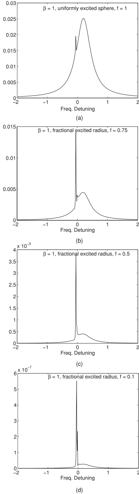
FIG. 4. The frequency spectrum of the power radiated by the medium, in arbitrary units, as a function of the frequency detuning, in units of n_0|\bar{\mu}|^2\beta/(3\hbar) , for \beta = 1 , with (a) f = 1 (uniform initial excitation); (b) f = 0.75 ; (c) f = 0.5 ; and (d) f = 0.1 .
