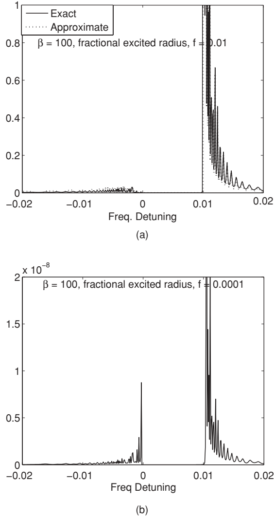
FIG. 6. Same as Figs. 5(a), except (a) \beta = 100 , f = 0.01 and (b) \beta = 100 , f = 0.0001 .
