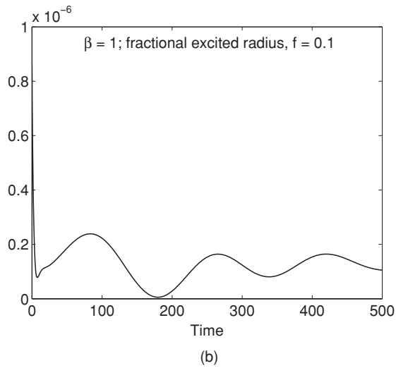
FIG. 7. The power radiated by the medium, in arbitrary units, as a function of time, in units of [n_0|\vec{\mu}|^2\beta/(3\hbar)]^{-1} , for \beta = 1 with (a) f = 1.0 and (b) f = 0.1 .
