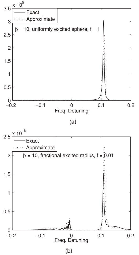
FIG. 5. Same as Fig. 4(a), except (a) \beta = 10 , f = 1 and (b) \beta = 10 , f = 0.01 .
