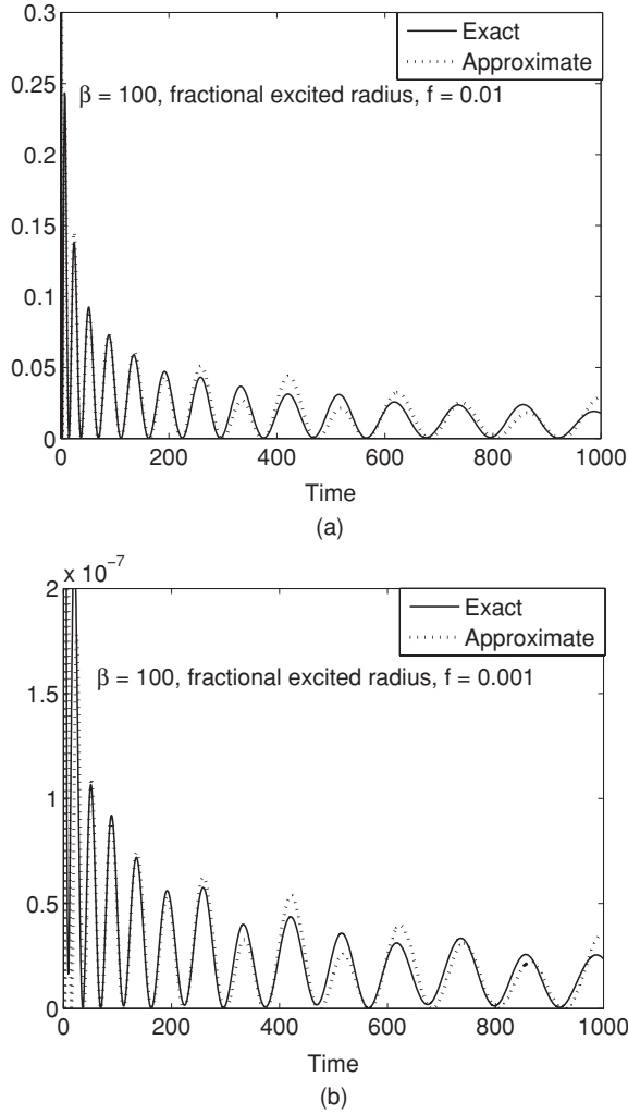
FIG. 9. Same as Figs. 7(a) and 7(b), except (a) \beta = 100 , f = 0.01 and (b) \beta = 100 , f = 0.001 .
