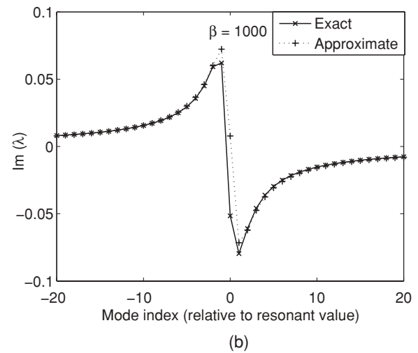
FIG. 2. (a) Decay rates and (b) frequency detuning (from resonance) for the 40 fastest decaying modes, for \beta = 1000 , in units of n_0 \mu^2 \beta / (3\hbar) .
