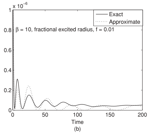
FIG. 8. Same as Figs. 7(a) and 7(b), except (a) \beta = 10 , f = 1.0 and (b) \beta = 10 , f = 0.01 .
