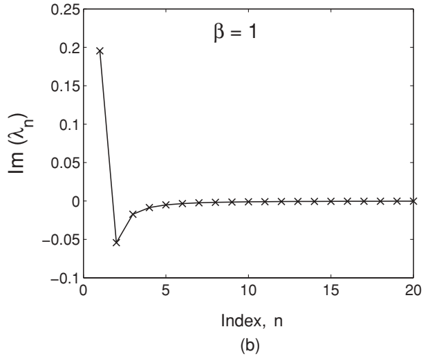
FIG. 1. (a) Decay rates and (b) frequency detuning (from resonance) for the 20 fastest decaying modes, for \beta = 1 , in units of n_0 \mu^2 \beta / (3\hbar) .
