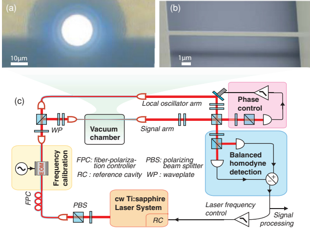
FIG. 1. (Color online) Optical and scanning electron micrographs of (a) a 16 \mu\text{m} radius microresonator and (b) a 100 nm \times 500 nm \times 15 \mu\text{m} strained SiN nanomechanical oscillator. (c) Schematic of the quantum-limited optical homodyne detection scheme. The samples are mounted in a vacuum chamber. A continuous wave (cw) titanium sapphire laser emitting at \lambda = 850 nm is fiber coupled.
