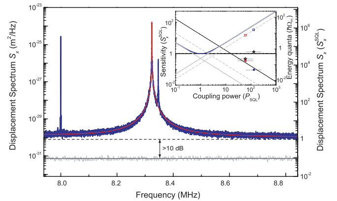
FIG. 4. (Color online) Shot-noise limited imprecision more than 10 dB below the SQL. The total measurement imprecision is approximately at the SQL. The shot-noise level (gray, lower line), however, lies >10 dB lower at S_x = 0.09 \times S_x^{\text{SQL}} or (250 \text{ am}/\sqrt{\text{Hz}})^2 . Inset: Sensitivity versus normalized optical input power. Full (dashed) gray lines mark shot noise and QBA for an ideal, lossless measurement (for an impedance-matched cavity). The solid blue line shows the total sensitivity. Stars mark the full imprecision for the spectra shown in Figs. 3 (inset) and 4 with different thermorefractive noise levels (owing to different optomechanical coupling). The measured shot-noise limited imprecision (squares) lies far below the value of the SQL, reaching 0.09 \times S_x^{\text{SQL}} for P_{\text{in}} = 130 \times P_{\text{SQL}} . The corresponding QBA noise (empty squares) is estimated to contribute n_{\text{QBA}} \approx 20 noise quanta. The full line (black) fits the measured shot-noise contribution.
