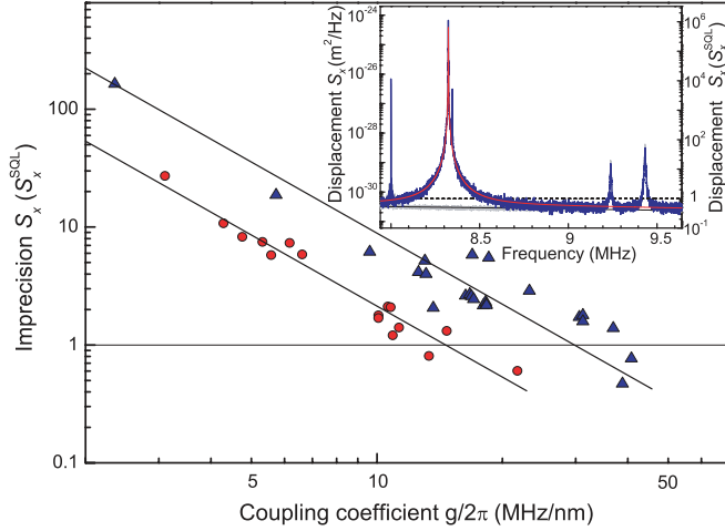
FIG. 3. (Color online) Optical measurement of nanomechanical motion with an imprecision below the SQL. The total measurement imprecision for an 8.3 MHz nanomechanical oscillator ( 4 \times 10^{-15} kg), using P_{\text{in}} = 1 \mu\text{W} (triangles) and P_{\text{in}} = 8 \mu\text{W} (circles), reduces with increased optomechanical coupling g/2\pi according to Eq. (3). Both power levels allow an imprecision below the SQL, achieving a best value of S_x = 0.47 \times S_x^{\text{SQL}} . Inset: Spectrum with the lowest imprecision at an input power of 1 \mu\text{W} (calibration marker at 8 MHz, first-order in-plane mode of the string at 8.4 MHz, and mechanical modes of the optical microresonator at >9 MHz).
