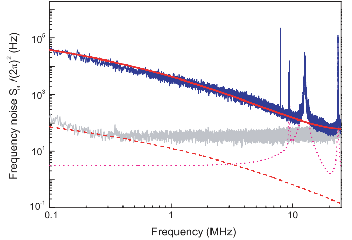
FIG. 2. (Color online) Frequency noise background of the microresonator. The measured equivalent frequency noise caused by shot noise (gray lower spectrum) lies far below the predominant broadband noise. The latter is due to thermorefractive cavity frequency noise according to Eq. (2) (thick red line, no adjustable parameters, also includes the measured shot noise). For a bath temperature of 30 K, a 25 dB reduction of thermorefractive noise is expected (dashed line). The mechanical modes of the microresonator (dotted line) have negligible off-resonant contributions (8 MHz: calibration marker).
