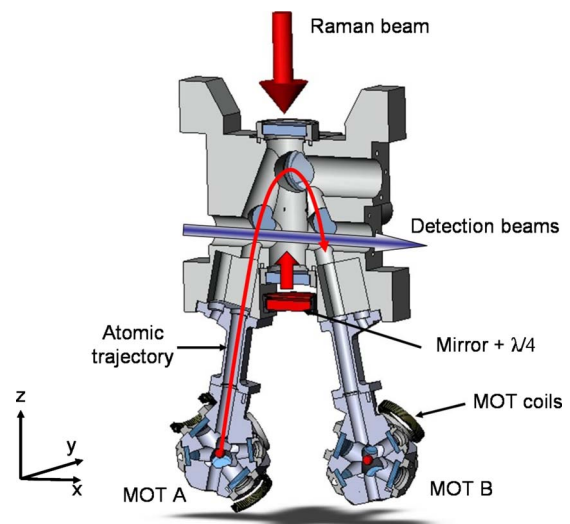
FIG. 1. (Color online) Scheme of the vacuum chamber showing the two MOTs, the interferometer zone and detection probe. The total dimensions of the system are 30 \times 10 \times 50 cm 3 .
