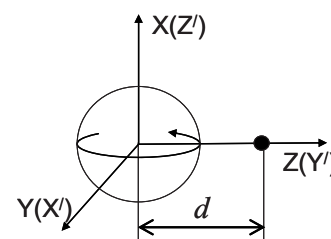
FIG. 1. The coordinate systems used in calculations and the original FM interacting with the defect (blackened small sphere).
