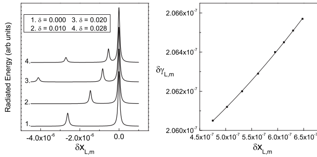
FIG. 2. Scattered power for different distance parameter \delta = (d - R_0 - R_d)/R_0 (left); relative broadening versus frequency shift of the |m|=1 resonance revealed through varying distance d (right). The line shows a fit with a quadratic polynomial.
