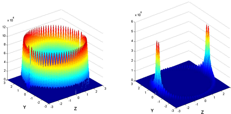
FIG. 3. (Color online) Internal field intensity of the microsphere in the YZ plane at the frequency of the standard Mie resonance (left) and the defect-induced resonance (right).
