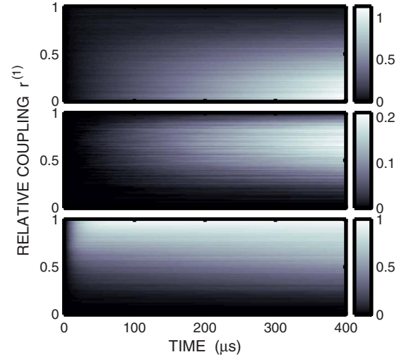
FIG. 6. (Color online) Average cumulative number of quantum jumps per ensemble member for each decay channel in the weak ion-cavity coupling regime. From above: C_S^{(1)} , C_S^{(2)} , and a . Parameters: \Delta/\Delta_0=100 , \kappa/\kappa_0=0.1 .
