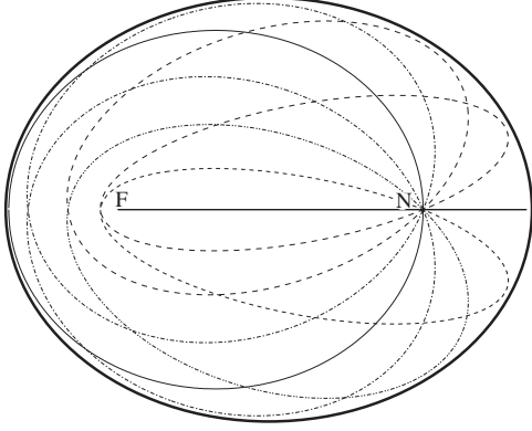
FIG. 2. The caustic (thick solid line) for the Kepler problem is an ellipse. Classically allowed orbits with the same energy, the same center of force F and a common starting point N have to lie inside this critical ellipse.
