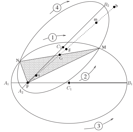
FIG. 1. Lambert's projection of elliptic motion to collinear motion. Shown are two ellipses with the same lengths of the semimajor axes \frac{1}{2}A_1B_1 = \frac{1}{2}A_2B_2 and a common focus located at F . The centers of the two ellipses are denoted by C_1 and C_2 . Lambert's lemma 24 allows to relate the motion from N to M on both ellipses to a common collinear motion on the degenerate linear ellipse Fb , where the points n and m are chosen such that the time of flight (TOF) along nm equals the TOF along the elliptical arc NM on the first ellipse. On the second ellipse the TOF along the arc NB_2M equals the TOF along nbm . The points n and m are found by marking the point G halfway between N and M . Then the major axis Fb = A_1B_1 = A_2B_2 of the linear ellipse is drawn starting at F and running through G . On this line the point g is placed at the distance Fg = \frac{1}{2}(FN + FM) . Finally n and m are given by the intersection points of a circle around g with radius GN = GM . This construction shows that the sum of the lengths of the shaded triangle \alpha_{\pm} = FN + FM \pm NM is equal to \alpha_{\pm} = Fn + Fm \pm nm . The fictitious collinear motion goes back to Lambert and can be pictured as the limit of an elliptic motion with extremely small semiminor axis b . The eccentricity approaches one from below in such a way that the moving particle turns around at F with very high but of course still nonrelativistic velocity.
