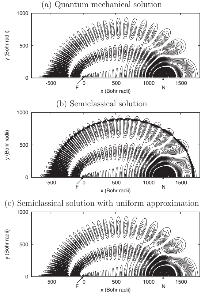
FIG. 4. Contour plot of |G^{(3)}(\mathbf{r}, \mathbf{r}'; E)|^2 with “principal” quantum number \nu=29.2 and center of force F at the origin. The initial position vector N at \mathbf{r}'=(1232, 0, 0) Bohr radii is located on the x axis, the final position vector \mathbf{r} is varied in the x, y plane.
