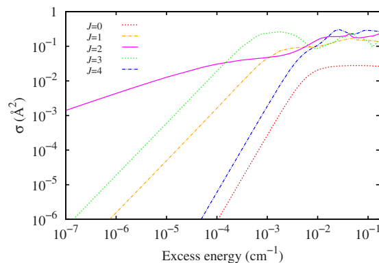
FIG. 8. (Color online) Near-threshold behavior of individual partial-wave contributions to the 11u \rightarrow 21l inelastic excitation cross section, from close-coupling calculations, as a function of the excess energy above the threshold for excitation.
