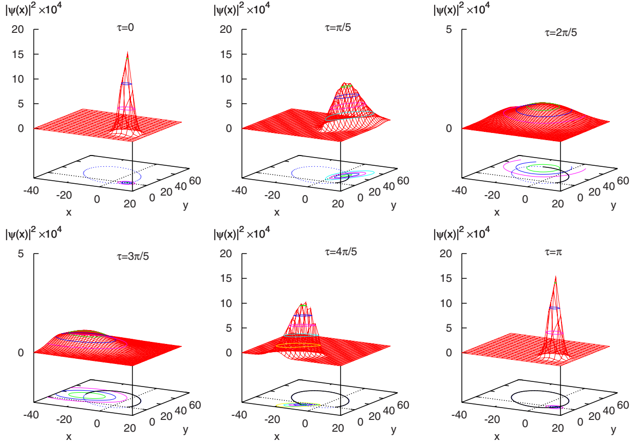
FIG. 1. (Color online) Fictitious time propagation of the initially Gaussian wave packet (41) located at \mathbf{x}_0=(8,0,0) with the momentum \mathbf{p}_0=(1,2,0) plotted in the plane z=0 . The classical Kepler ellipse with the same initial conditions is indicated by the dotted curve on the bottom of each panel. For time resolved comparison, that part of the ellipse that has been traversed by the particle so far in each plot is shown by a solid black line. Although the Gaussian wave packet does not stay Gaussian during the period it follows in general the classical path and is recovered after one period \tau=\pi , indicating the periodicity of the wave packet. Lengths are given in scaled atomic unit na_0 with a_0 the Bohr radius [see Eq. (10)].
