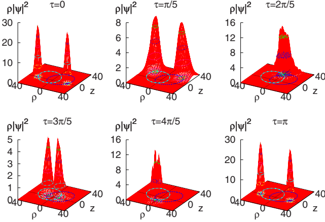
FIG. 2. (Color online) Fictitious-time propagation of GWP (57) with magnetic quantum number m=0 . The part on the negative \rho axis is obtained by reflecting the positive part at the z axis. The wave packet runs along the classical Kepler ellipse with the corresponding initial values. For details see text.
