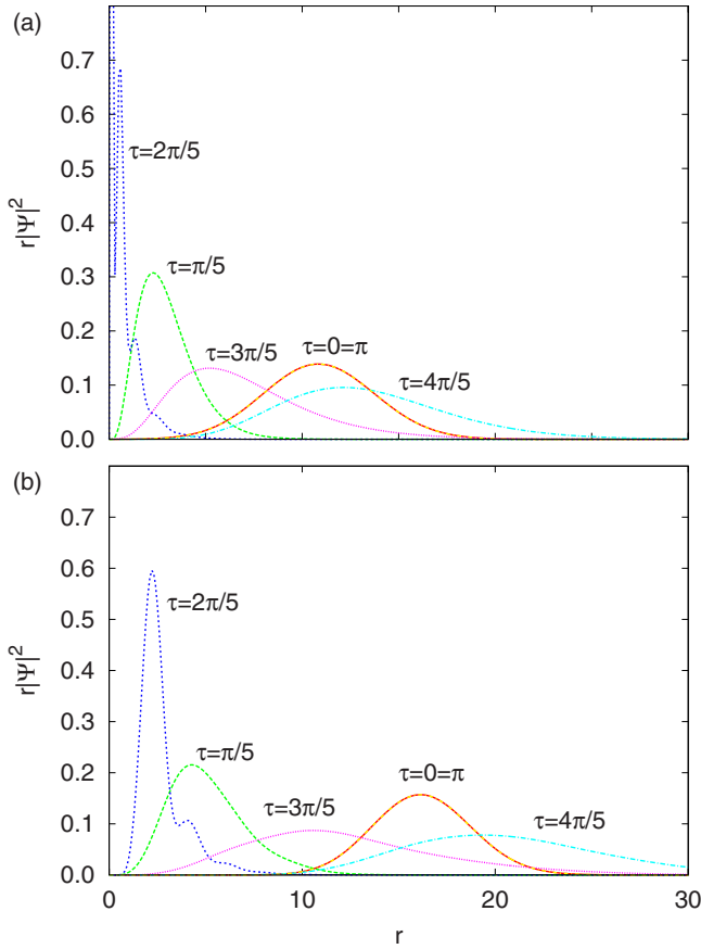
FIG. 3. (Color online) Fictitious-time propagation of the wave function (69) with \psi(r) given by the Gaussian (68) with r_0=10.0 , p_{r_0}=-0.5 , and \sigma=3.0 for angular momentum quantum numbers (a) l=0 , m=0 and (b) l=5 , m=0 . An interference pattern is observed at the turning points at approximately \tau=2\pi/5 in both panels. The initial wave function is expanded in N=10\,000 basis states [Eq. (62)] with \epsilon=0.2 .
