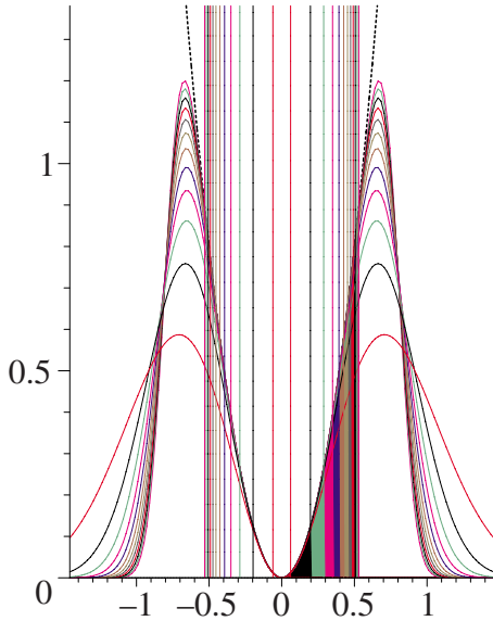
FIG. 7. (Color online) Integrated focal intensity profiles \bar{I}(x,0) of Hermite-Gauss beams comprising up to 23-rd order modes (compare Fig. 2), and their 0.74%-deviation marks d_{2J+1} , which lie at relative positions d_{2J+1}/d_1=1.00, 3.24, \dots, 8.70 from the origin (compare Table I) (same units as in Fig. 2; in contrast to Fig. 5 total beam power normalized to unity, but Rayleigh lengths z_{Rx} readjusted such that all higher-order superpositions match up with curvature of the first mode case \Psi_1 ; see text).
