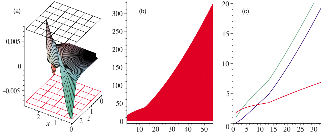
FIG. 8. (Color online) Left: Behavior of the relative deviation of the intensity distribution \Delta \bar{I} from zero as it approaches the 0.74%-deviation marks (top and bottom grid). Here, \Delta \bar{I}_{23} is shown for the crossed configuration of two laser beams traveling along the z and x axes, respectively. The value of the Rayleigh length z_{R_x} at which we find that the oscillatory behavior of \Delta \bar{I} along a constant radial perimeter just exhausts the upper and lower limits set by the deviation marks allows us to determine the associated value of z_{\min} . The latter is plotted as a function of maximum mode number, in the middle panel (the filled-in red area is the forbidden area of too tightly focused beams). The values of z_{\min}(2J+1) in turn determine the positions of the turning points 0.57\sqrt{2J+1}w_{0x} (top green line), the positions of the deviation points d_{2J+1} (middle blue line), and the minimal beam widths w_{0x}(2J+1) (bottom red line), depicted in the right panel in units of the laser's wavelength \lambda_L .
