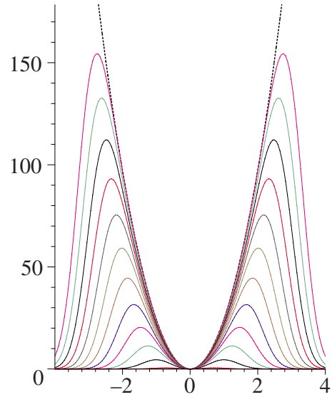
FIG. 5. (Color online) Integrated focal intensity profiles \bar{I}(x, 0) of Hermite-Gauss beams comprising up to 23rd-order modes; compare Fig. 2 (same units as in Fig. 4; total beam power adjusted such that all profiles have same curvature at origin as the dotted line parabola).
