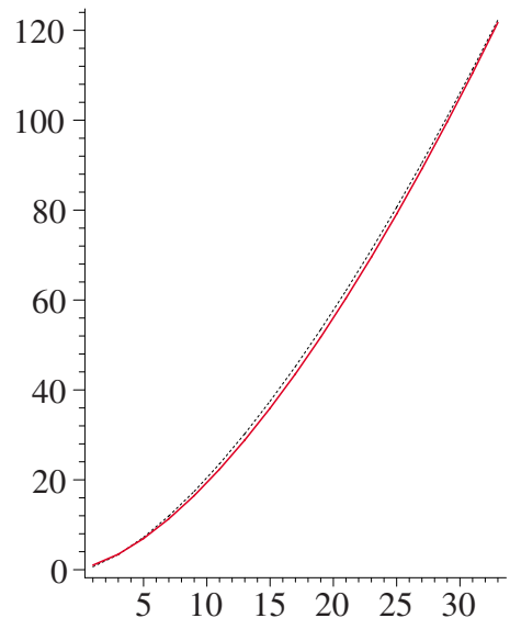
FIG. 6. (Color online) The increase in total beam power needed to achieve the power compensation described in the text and displayed in Fig. 5 as a function of mode number (solid red line) scales approximately like (20/31)(2J+1)^{3/2} (dotted black line).
