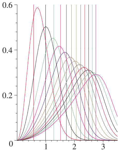
FIG. 4. (Color online) Integrated focal intensity profiles \bar{I}(x, 0) of Hermite-Gauss superposition beams comprising up to 23rd-order modes; compare Fig. 2 (same units as in Fig. 2; vertical bars mark location of position 0.57\sqrt{2J+1}w_{0x} , confirming harmonic oscillator scaling [35]).
