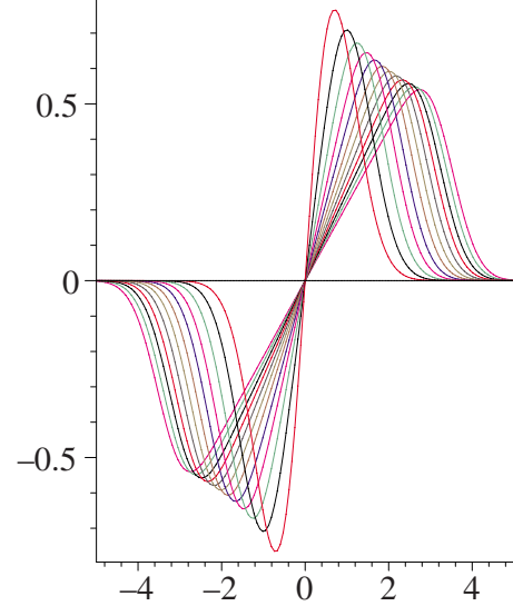
FIG. 2. (Color online) Electric field profile E_{2J+1}(x,0,0) at focal cross section of Hermite-Gauss beams comprising superpositions of up to 23rd-order odd modes (i.e., 2J+1=1,3,\dots,23 ; x axis in units of beam waist w_{0x} , total cross-sectional beam power normalized to unity, Rayleigh lengths kept constant, \epsilon_0\omega_L^2/2 set to unity).
