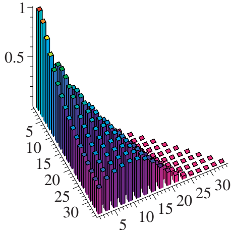
FIG. 3. (Color online) Amplitude coefficients c_{2j+1} of Hermite-Gauss superpositions \Psi_{2j+1} of up to 33rd-order modes ( 2J+1 = 1, 3, \dots, 33 ).
