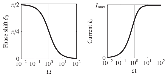
FIG. 2. The phase between current in the conducting loop and the driving field (left) and the induced current (right) as a function of the frequency of the driving field. Note that at low frequencies, the phase-induced current lags \pi/2 behind the driving field. For the simulations in Fig. 3, \Omega=4 .
