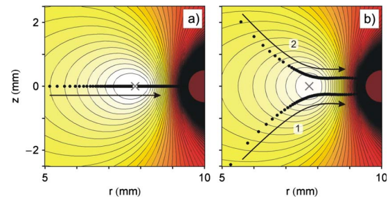
FIG. 3. (Color online) The magnetic potential about the conducting loop showing the effect of the control parameters. The positions of the time-averaged trap minima are marked by the gray crosses, and the instantaneous zeros of the B field are denoted by the black dots. The trajectory that the minima follow is indicated by the numbered, black arrows. For these results, \omega=(2\pi)30 kHz, B_0=100 G. (a) No additional fields. (b) A dc quadrupole field, B_{\text{dcq}}=25 G \text{cm}^{-1} , is added.
