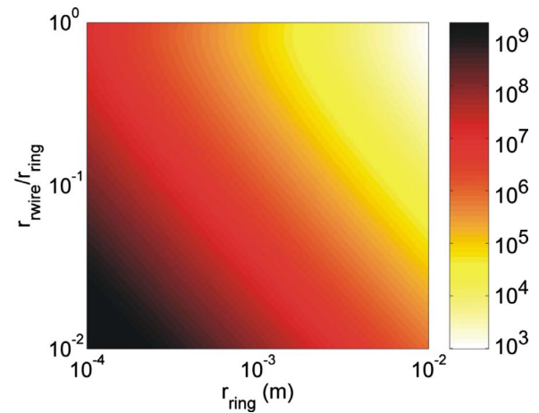
FIG. 5. (Color online) The scaling of drive frequency, \omega_{\text{drive}} \sim \omega = R/L , as a function of r_{\text{ring}} and r_{\text{wire}} . The y axis is presented as the ratio of the length scales in the range of experimental interest.
