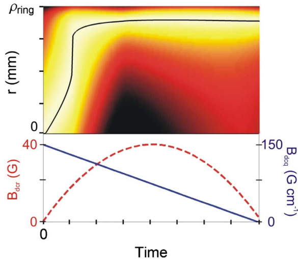
FIG. 4. (Color online) The transfer from the single quadrupole potential to a ring trap. The quadrupole field is reduced while a transverse bias field is applied to shift the zero of the quadrupole toward the ring radius. The top figure shows the potential along a radius parallel to the bias field as the applied fields vary in time, shown in the lower figure.
