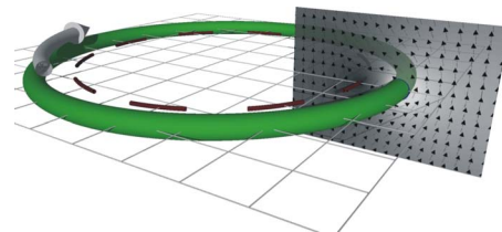
FIG. 1. (Color online) Schematic of the instantaneous vector fields for the system described in the text. The external bias field, increasing in magnitude, points upwards, while the induced current in the loop, indicated by the arrow, creates a field about the loop. The fields cancel at a radius inside the loop, indicated by the red, dashed circle. The gray scale in the field slice indicates field magnitude and arrows show the field direction.
