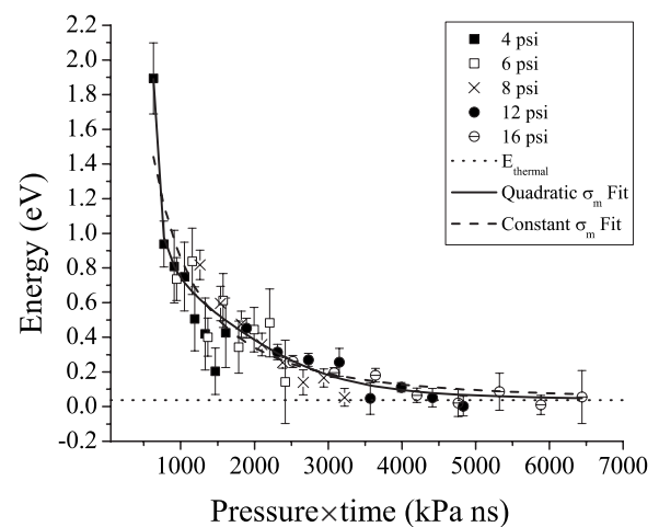
FIG. 5. Thermalization results—best fits for \sigma_m held constant and allowed a quadratic dependence shown with all of the DB results.
