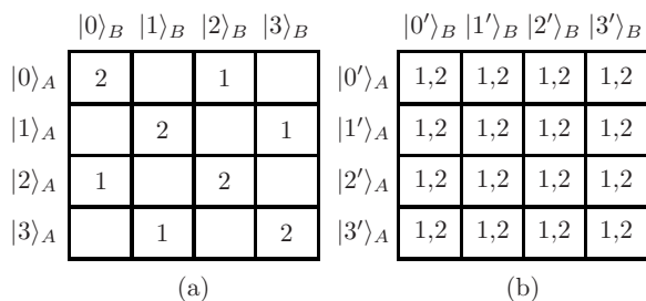
FIG. 1. Representation of the set of states given in Eq. (2). Alice’s basis states are denoted along the left side of each grid, Bob’s along the top. The numbers ( j ) inside the boxes indicate that the state ( |\Psi_j\rangle ) has the corresponding product state as a component. (a) For the bases of Eq. (2), it is easily seen that the states can be distinguished by LOCC, preserving Schmidt rank of 2 for all outcomes. (b) When viewed in other bases, the distinguishability may be far from obvious.
