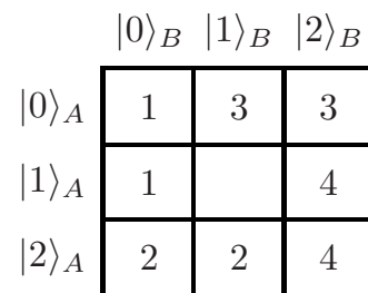
FIG. 7. Demonstration that theorem 3 does not provide a necessary condition. These product states can be distinguished (so R_j = 1 is preserved in all cases), but they cannot be completely partitioned by a cascading sequence. In fact, they cannot be partitioned even once into two nonempty subsets where the reduced density operators in one subset are orthogonal to all those in the other.
