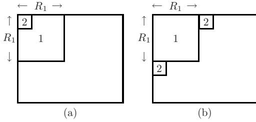
FIG. 8. Intuitive picture indicating how theorem 4 can be proved. The parts of this figure correspond to the two ways it can happen that \hat{\rho}_2 \hat{\rho}_1 \neq 0 (only selected components of |\Psi_2\rangle are shown). In either case, any individual measurements the parties can perform that preserve R_j leave the picture essentially unchanged, which means they have not distinguished. See Appendix A 3 for a detailed proof.
