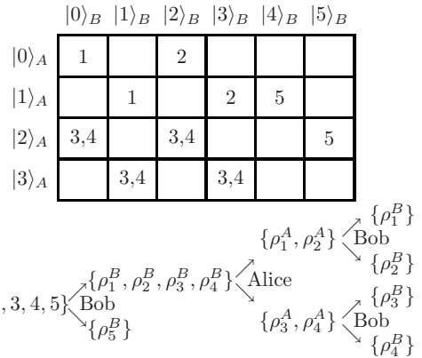
FIG. 6. Illustration of the procedure of cascading partitions for testing theorem 3, described in the text [the states are given in Eq. (16)]. Bob can separate out \{\rho_5^B\} since it is orthogonal to all the others, after which Alice can divide the remaining four into \{\rho_1^A, \rho_2^A\} and \{\rho_3^A, \rho_4^A\} . Then Bob can complete the partitioning.
