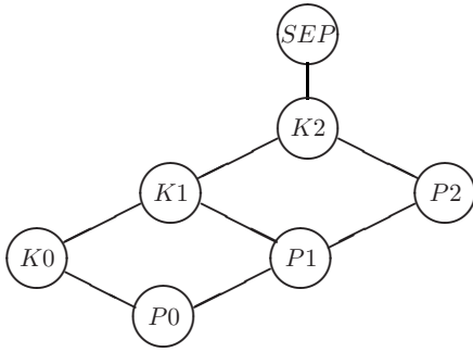
FIG. 2. Lattice diagram showing relationships between the various types of protocols discussed in the text. A connected path upward (downward) from one vertex, possibly passing through others, to a second vertex indicates that a sufficient (necessary) condition on the first implies the same for the second.
