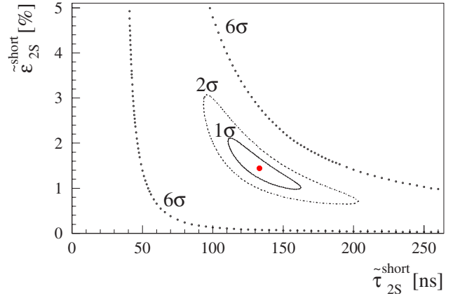
FIG. 3. (Color online) Relative population \tilde{\varepsilon}_{2S}^{\text{short}} (normalized to A_\alpha ) of the short-lived \mu p(2S) component versus its lifetime \tilde{\tau}_{2S}^{\text{short}} (without systematic corrections). The dot represents the best fit.
