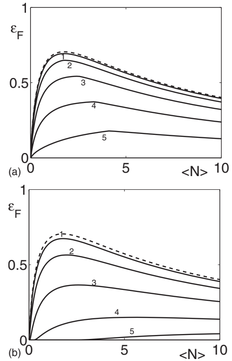
FIG. 5. The off-resonance interaction effect in the TWB case, both atoms in the ground state and g\tau=4.61 . (a) \Delta_A\tau=0 and \Delta_B\tau=0 (dashed line), 1, 2, 3, 4, 5. (b) \Delta_A\tau=\Delta_B\tau=0 (dashed line), 1, 2, 3, 4, 5.
