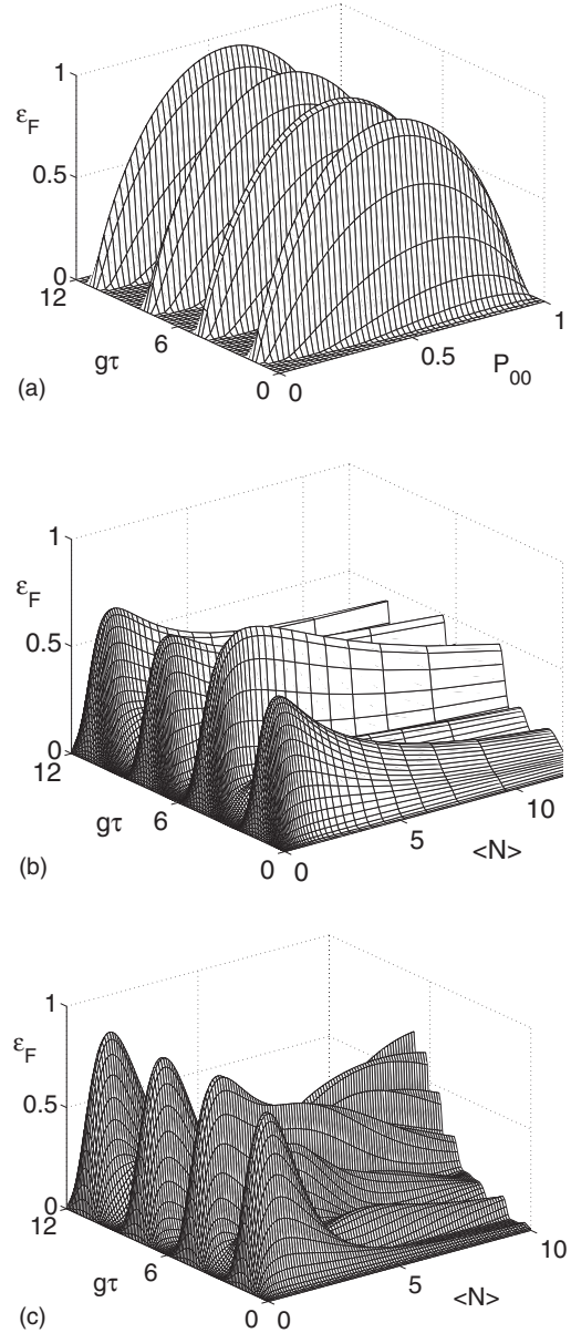
FIG. 2. Entanglement of formation \epsilon_F of the qubit systems as a function of the dimensionless time g\tau and the CV state parameter P_{00} (a) or the average number of photons \langle N \rangle (b,c) for the case of both atoms initially in the ground state. (a) TSS, (b) TWB, (c) TMC.
