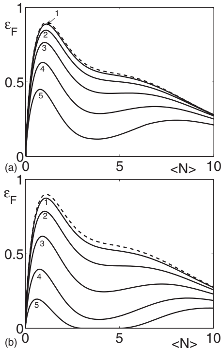
FIG. 4. The off-resonance interaction effect in the TMC case, both atoms in the ground state and g\tau=4.66 . (a) \Delta_A\tau=0 and \Delta_B\tau=0 (dashed line), 1, 2, 3, 4, 5. (b) \Delta_A\tau=\Delta_B\tau=0 (dashed line), 1, 2, 3, 4, 5.
