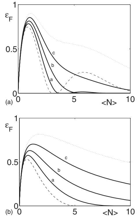
FIG. 7. The entanglement of formation \epsilon_F vs \langle N \rangle for a time g\tau of simultaneous presence of both atoms after the delayed injection of atom A. Atom A is prepared in the ground state and atom B in superposition states such that |B_1|^2 = 0 (dashed line), (a) 0.25, (b) 0.50, (c) 0.75, 1 (dotted line). (a) The TMC case with g\tau = 4.66 . (b) The TWB case with g\tau = 4.61 .
