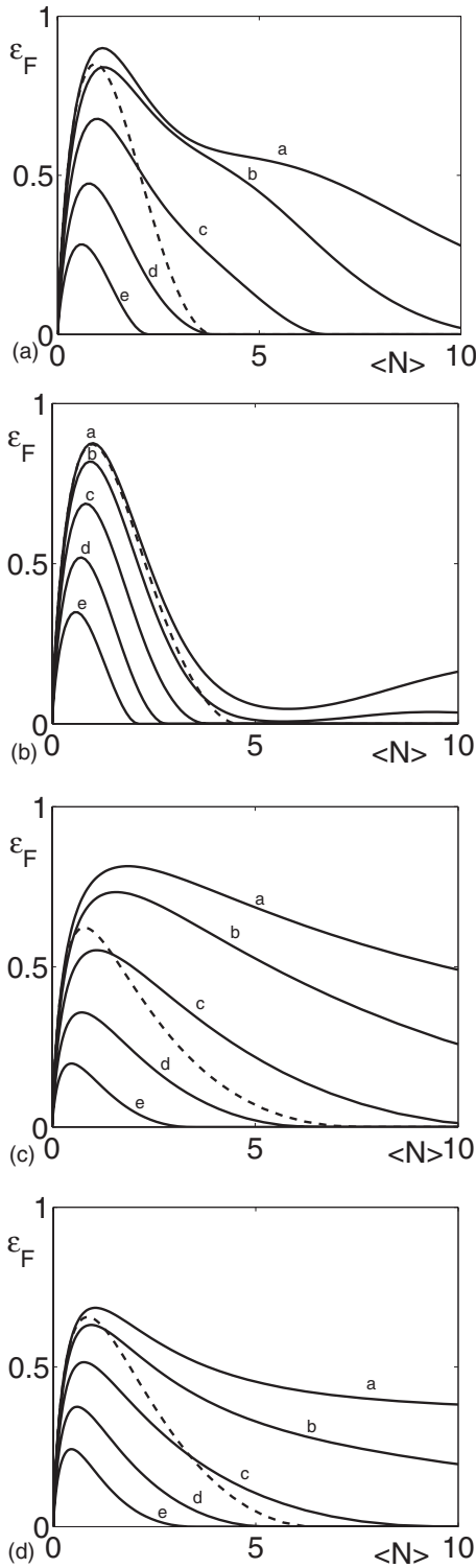
FIG. 6. The effect of different interaction times for \Delta_A = \Delta_B = 0 , and both atoms injected simultaneously in the ground state. In (a) the TMC case for g\tau_A = 4.66 and g\tau_B values (a) 4.66, (b) 4.4, (c) 4.2, (d) 4.0, (e) 3.8 and 1.56 (dashed line). In (b) the TMC case for g\tau_A = 11.01 and g\tau_B values (a) 11.01, (b) 10.8, (c) 10.6, (d) 10.4, (e) 10.2 and 7.85 (dashed line). In (c) the TWB case for g\tau_A = 4.61 and g\tau_B values (a) 4.61, (b) 4.4, (c) 4.2, (d) 4.0, (e) 3.8 and 1.56 (dashed line). In (d) the TWB case for g\tau_A = 11.03 and g\tau_B values (a) 11.03, (b) 10.8, (c) 10.6, (d) 10.4, (e) 10.2 and 7.85 (dashed line).
