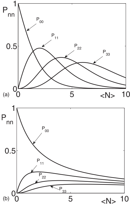
FIG. 1. The first four terms P_{nn} , n=0, \dots, 3 of the joint photon distribution of the state |x\rangle as a function of average photon number \langle N \rangle . (a) TMC, (b) TWB.
