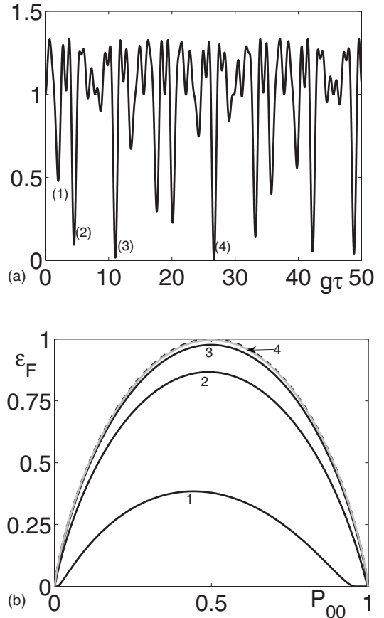
FIG. 3. (a) The function \lambda_4^{PT}(\frac{1}{2}, g\tau) + \frac{1}{2} as in Eq. (20) for the Bell-state case with both atoms in the excited state. (b) Entanglement of formation \epsilon_F vs P_{00} for TSS states compared to Von Neumann entropy (dashed line) for some values of g\tau , corresponding to the following numbered minima: (1) 2.03, (2) 4.53, (3) 11.07, (4) 26.68.
